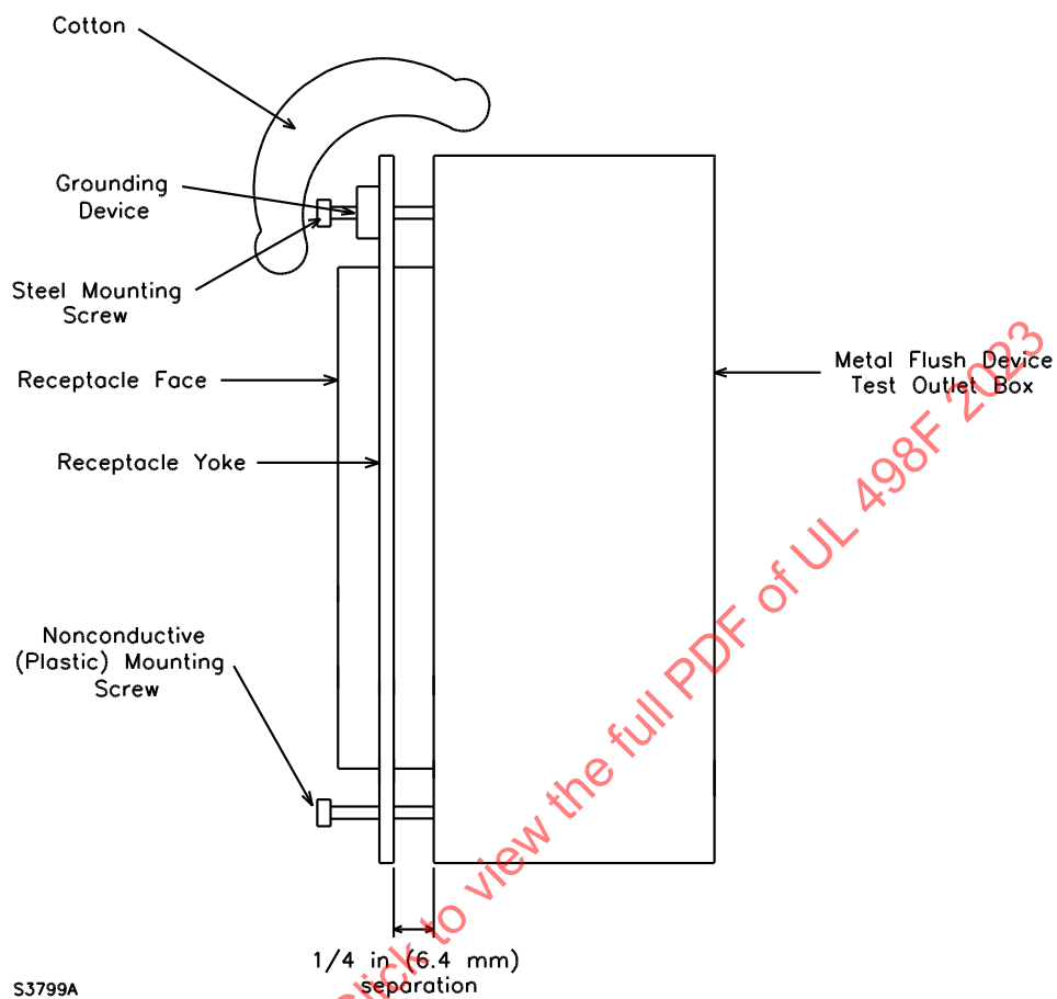
Figure 77.1 Fault Current Assembly
