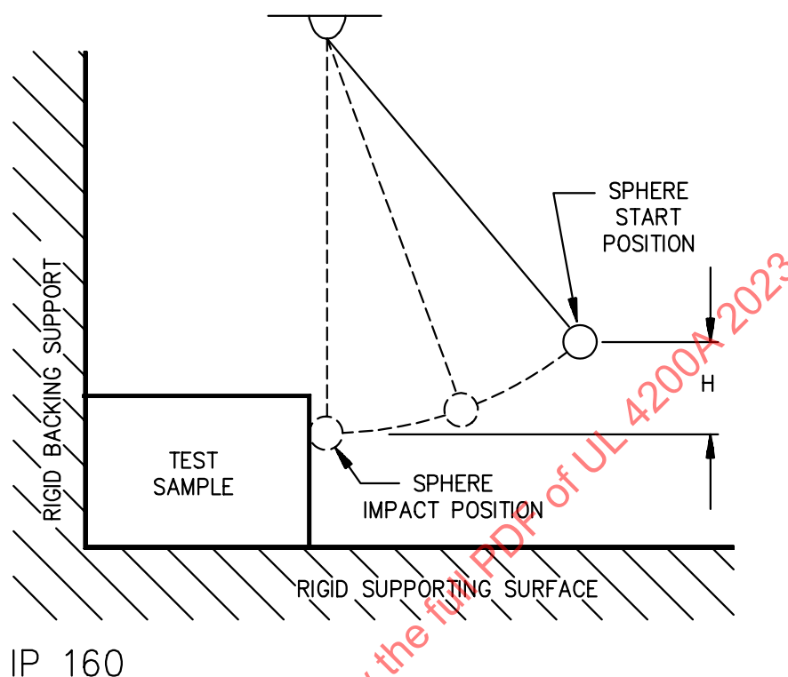
Figure 6.2 Impact test
