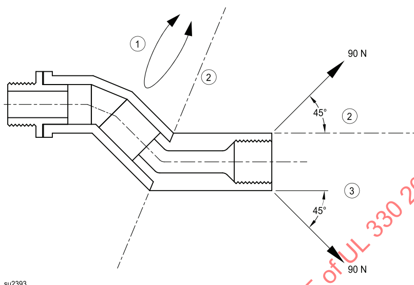
Figure 17.3 Application of Test Force on Compound Swivel with 45° Outlet
