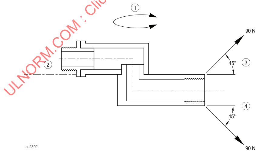
Figure 17.2 Application of Test Force for Compound Swivel
