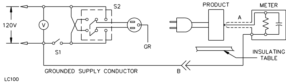
Figure 34.1 Leakage current measurement circuit
