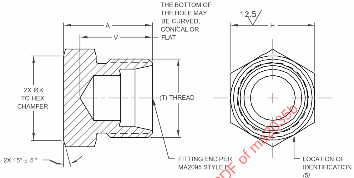
FIGURE 1 - PLUG
