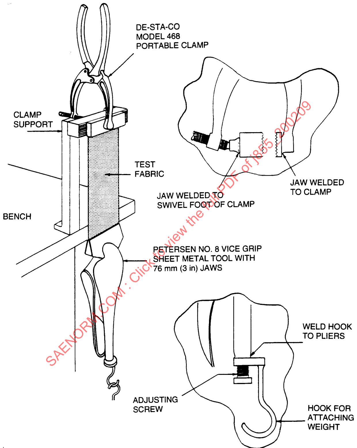
FIGURE 1—CLAMP AND FIXTURE ASSEMBLY FOR STRETCH AND SET OF TEXTILES
