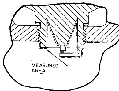
FIG. 3 - SPARK PLUG AREA
