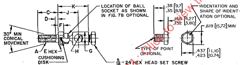
FIG. 7A—STYLE 1
