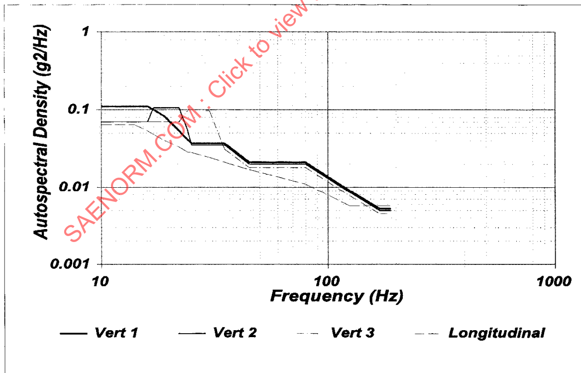
FIGURE 2 - VIBRATION SPECTRA FOR RANDOM VIBRATION TEST
