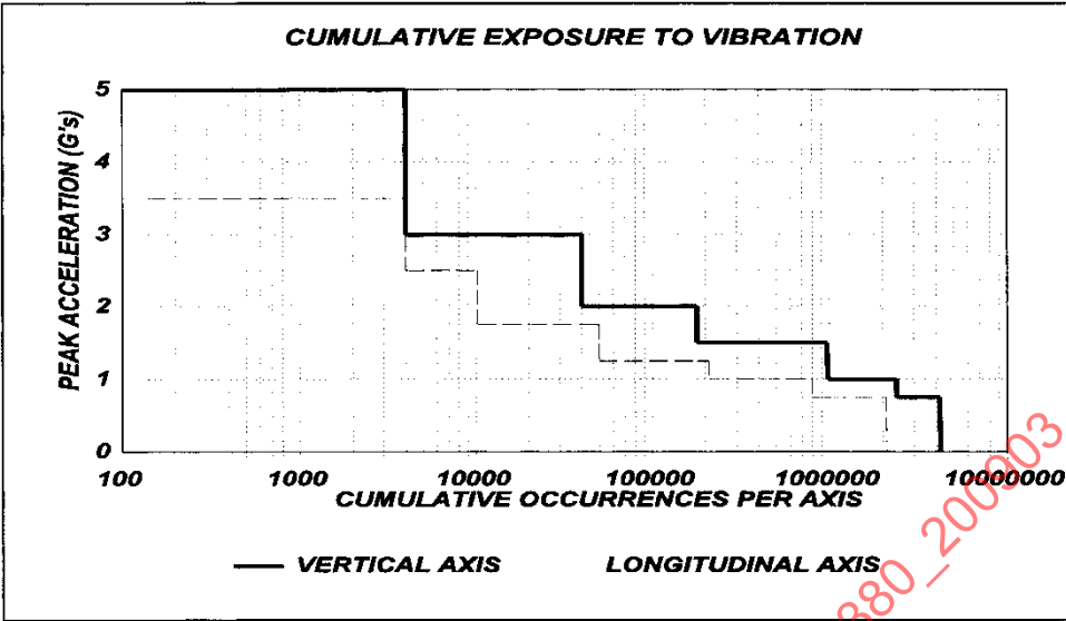
FIGURE 1 - CUMULATIVE VIBRATION ENVELOPES
