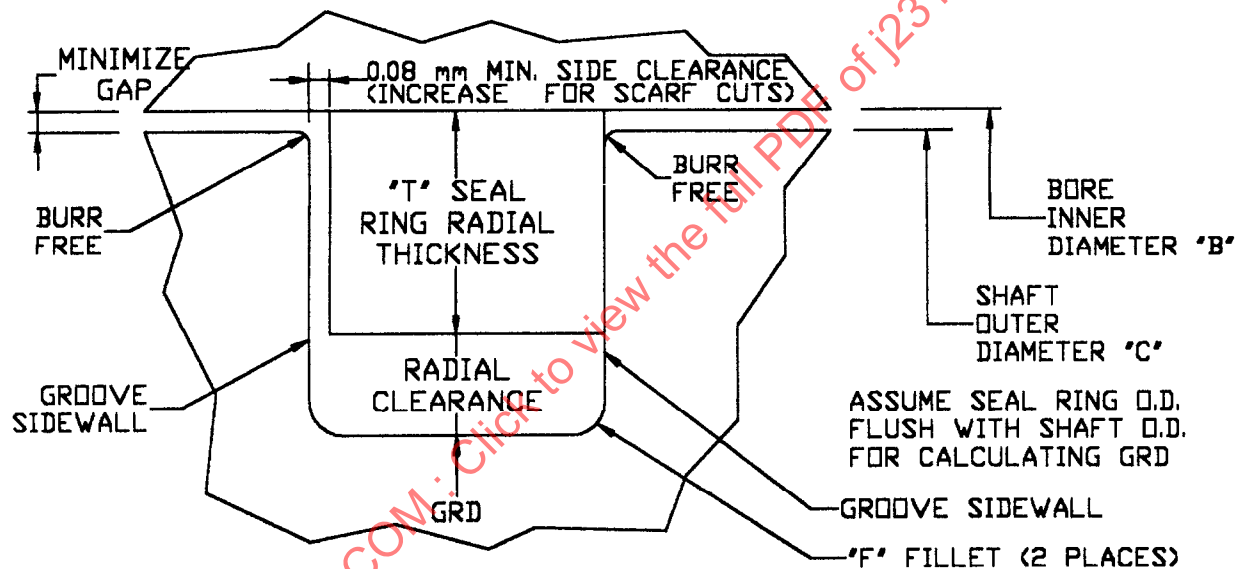
FIGURE 6 - GROOVE DIAMETER AND SIDE CLEARANCE
