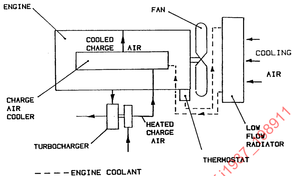
FIGURE A2 - "Low Flow Coolant" Vehicle Charge Air Cooler System
