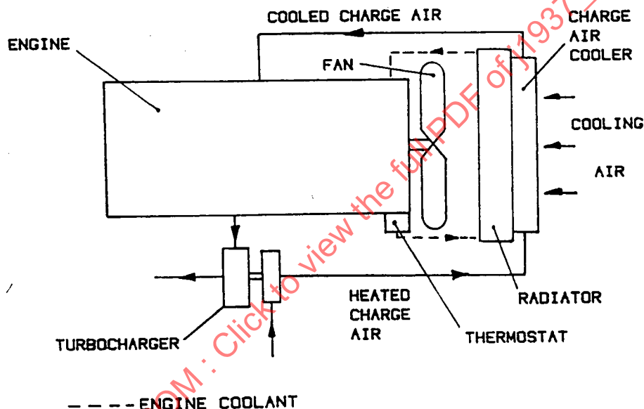
FIGURE A1 - "Air-to-Air" Vehicle Charge Air Cooler System
