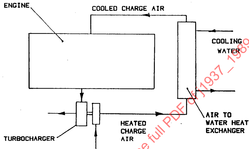
FIGURE A4 - "Air-to-Water" Test Cell Charge Air Cooler System
