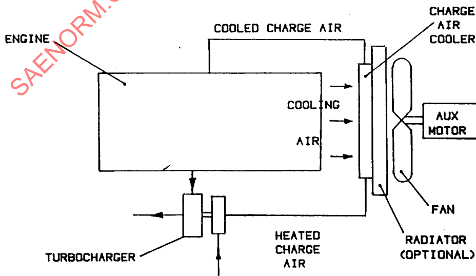
FIGURE A7 - "Air-to-Air (Auxiliary Fan)" Test Cell Charge Air Cooler System
