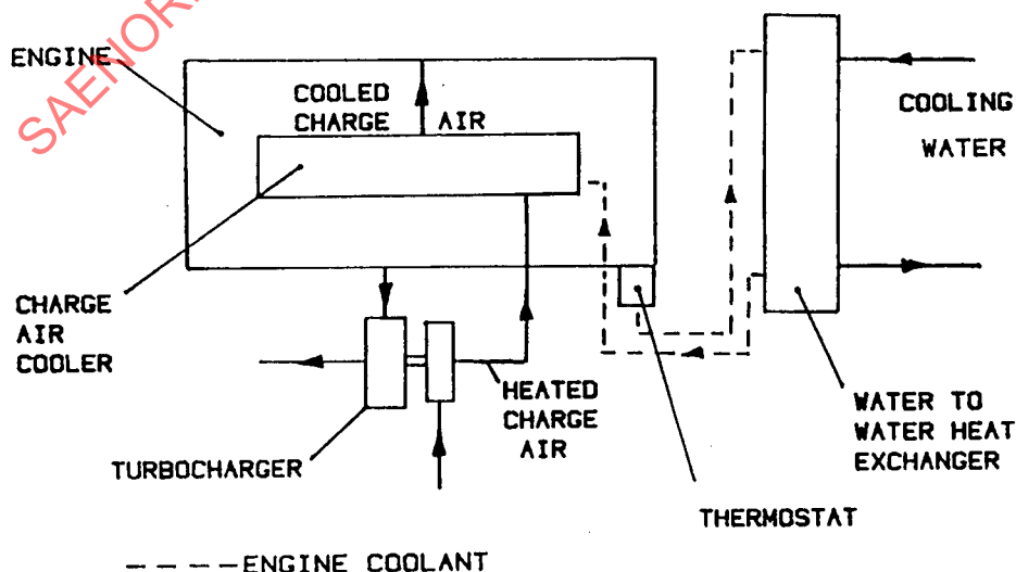
FIGURE A3 - "Water-to-Water" Test Cell Charge Air Cooler System
