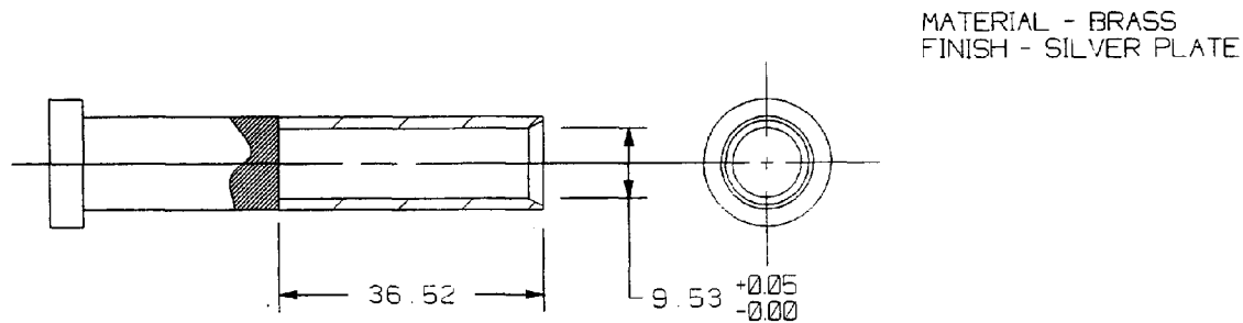
FIGURE 6—SOCKET TERMINAL
