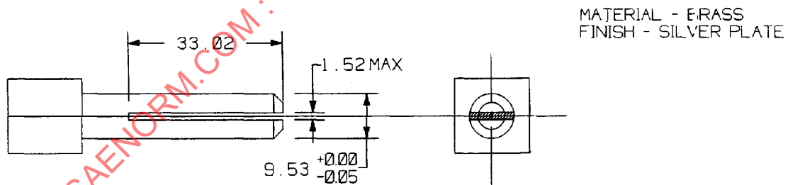
FIGURE 5—PIN TERMINAL
