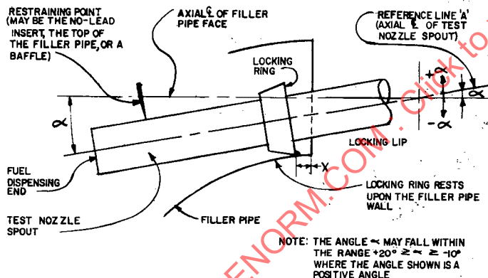
FIG. 1A—SAE J1114 TYPE FILLER PIPE (NORMAL RESTING POSITION)
