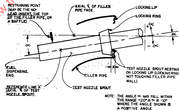
FIG. 2A—SAE J829b TYPE FILLER PIPE (NORMAL RESTING POSITION)
