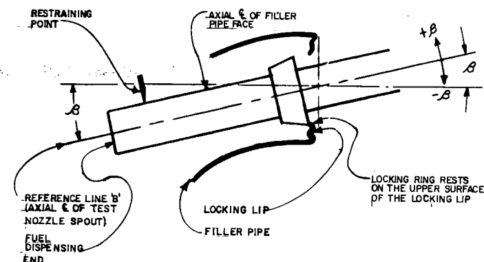
FIG. 2B—SAE J829b TYPE FILLER PIPE (INSERTION POSITION)
