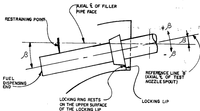
FIG. 1B—SAE J1114 TYPE FILLER PIPE (INSERTION POSITION)
