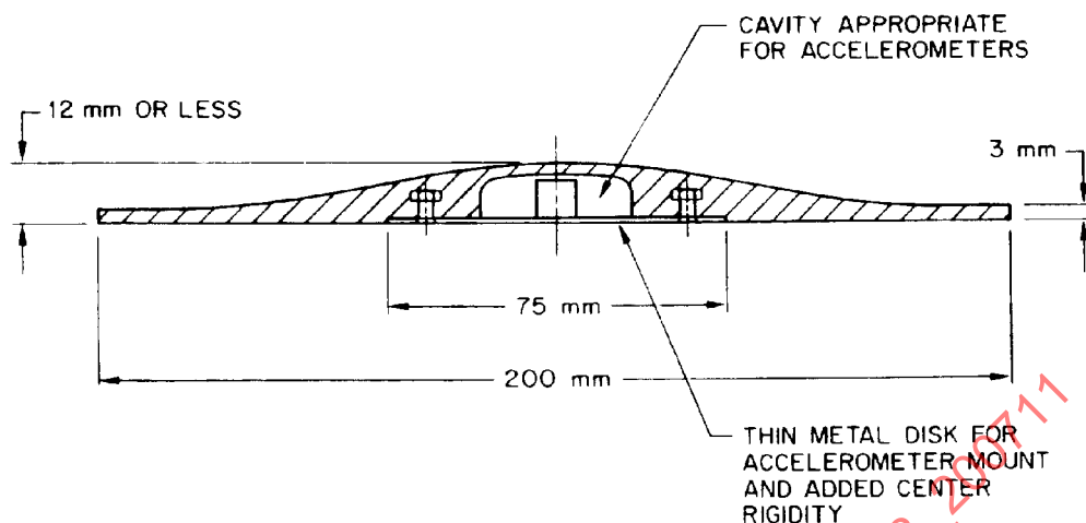
FIGURE 3—SUGGESTED DESIGN FOR SEMIRIGID DISC OF APPROXIMATELY 80 TO 90 DUROMETER (A-SCALE) MOLDED RUBBER, PLASTIC, ETC.
