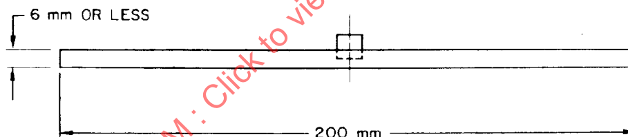
FIGURE 2—SUGGESTED DESIGN FOR RIGID DISC WITH ACCELEROMETER ASSEMBLY BONDED AT CENTER
