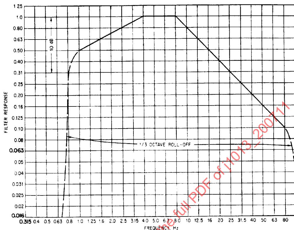
FIGURE 4—FILTER RESPONSE IN VERTICAL MODE, a_z
