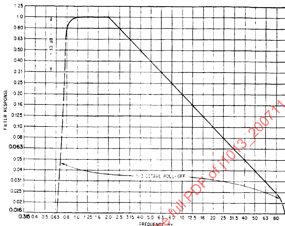
FIGURE 5—FILTER RESPONSE FOR a_x AND a_y
