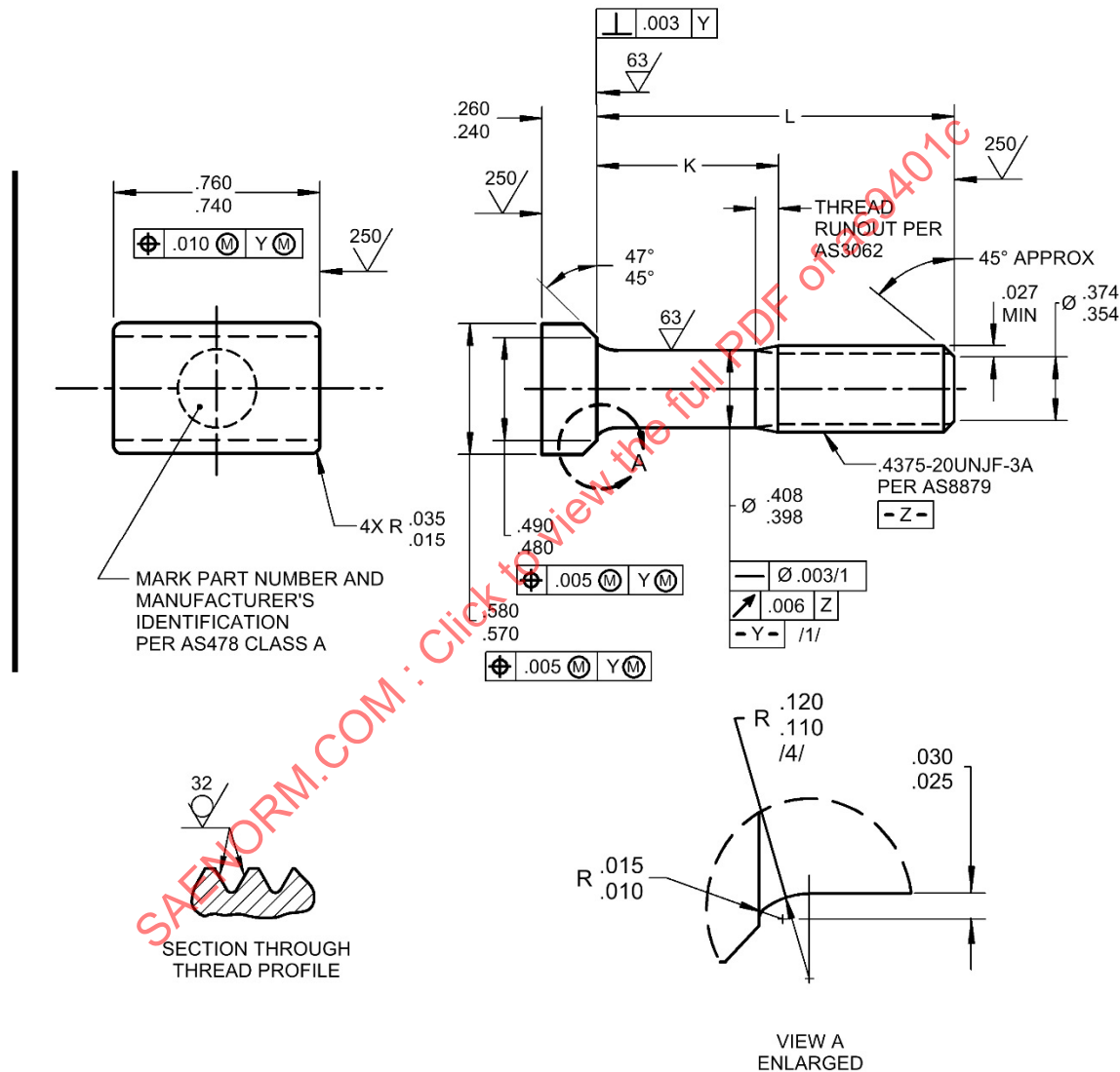
FIGURE 1 - BOLT
