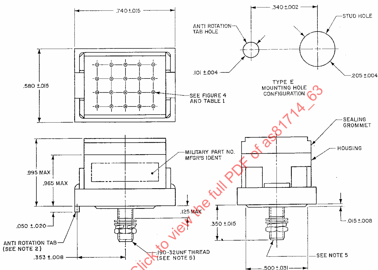
FIGURE 1. STUD MOUNTING TYPE S.
