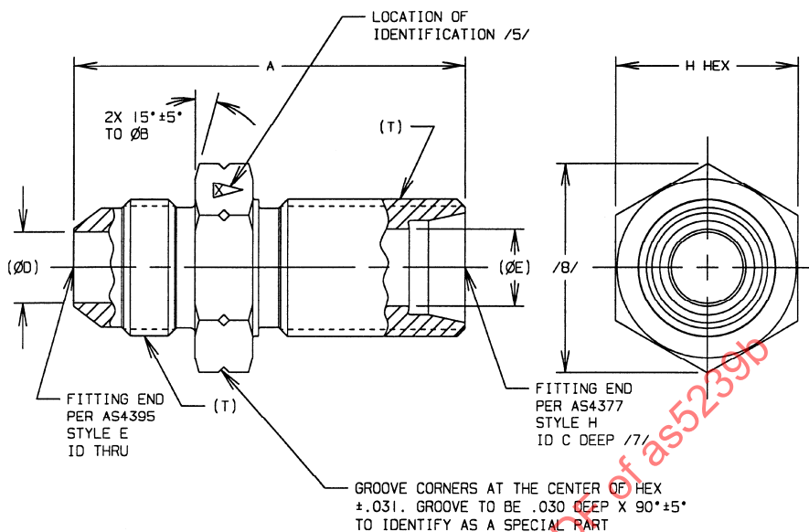
FIGURE 1 - FITTING, ADAPTER
