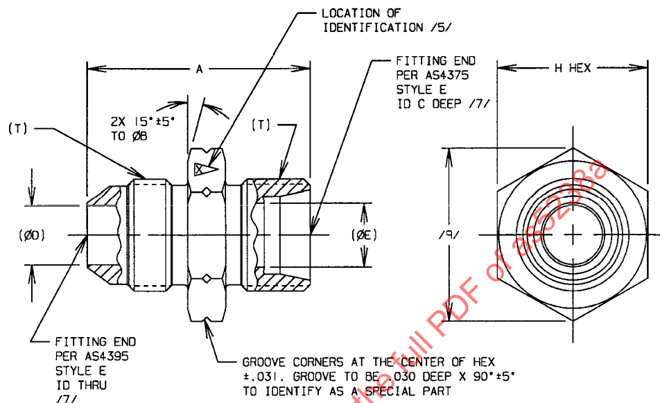
FIGURE 1 - FITTING, ADAPTER
