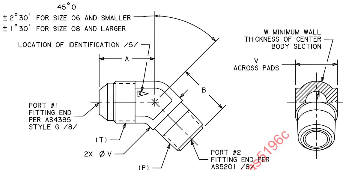
FIGURE 1 – FITTING, ELBOW, 45° TABLE 1 – DIMENSIONS
