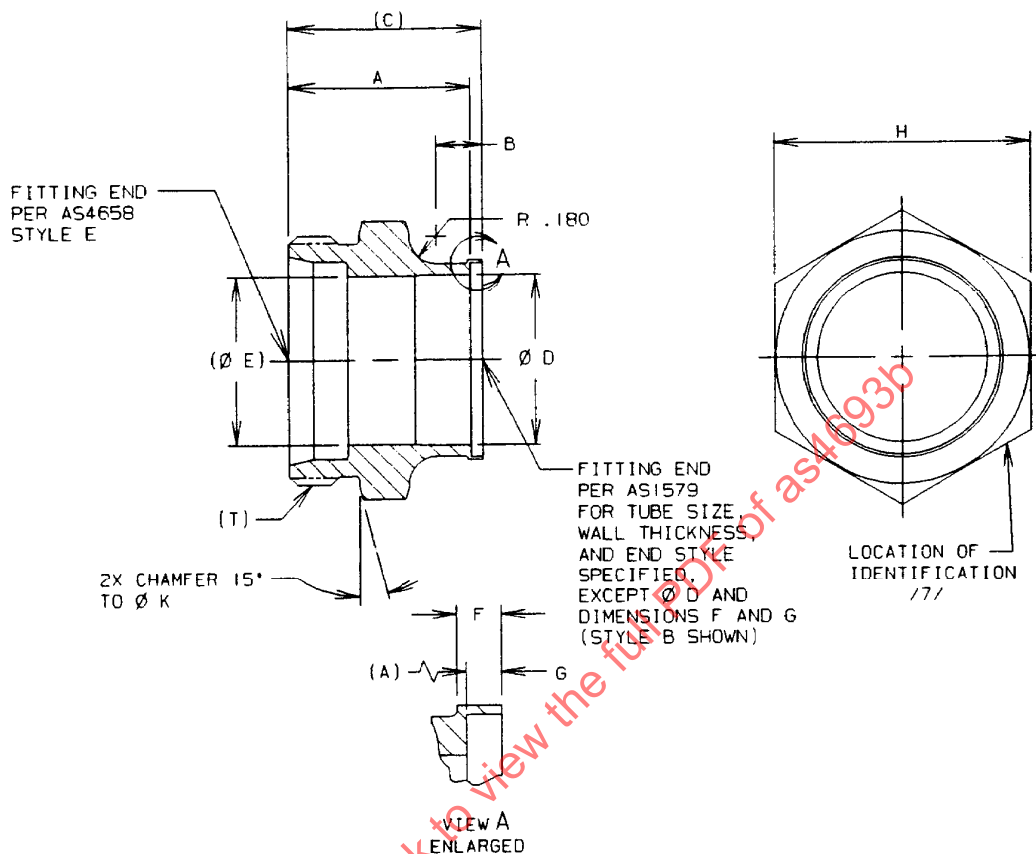
FIGURE 1 - UNION, TUBE END
