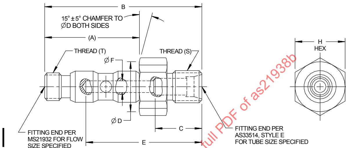
FIGURE 1 - BOLT, CLUSTER FITTING, SINGLE PORT, FLARELESS, DIMENSIONS AND CONFIGURATION
