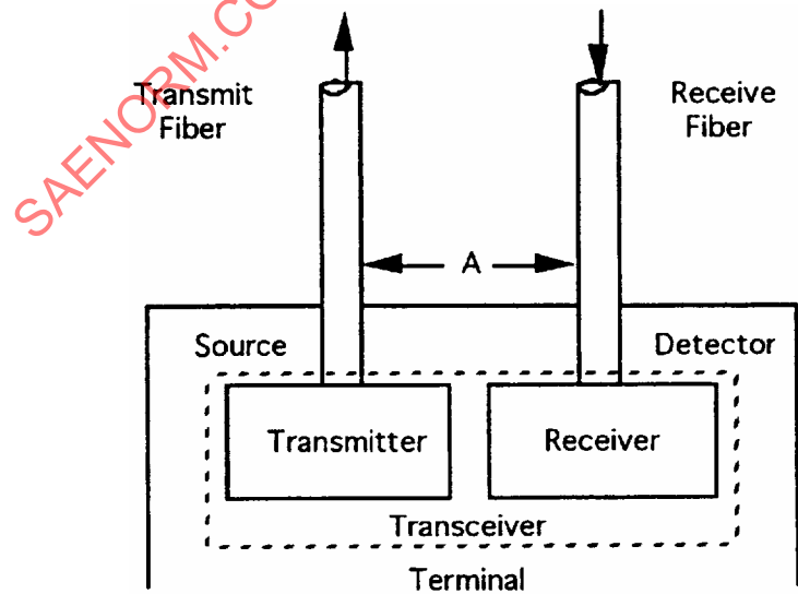
FIGURE 9 - Data Bus Interface with Pigtailed Fibers
