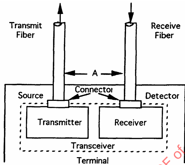
FIGURE 10 - Data Bus Interface with Connectorized Components
