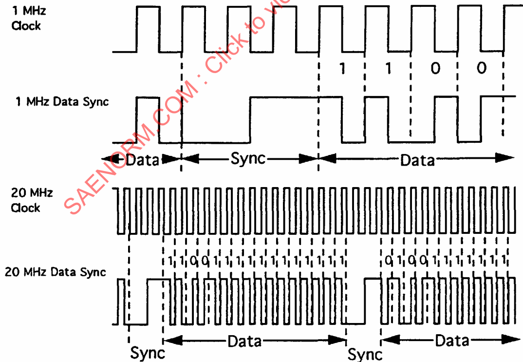
FIGURE 5 - Data Word Sync
