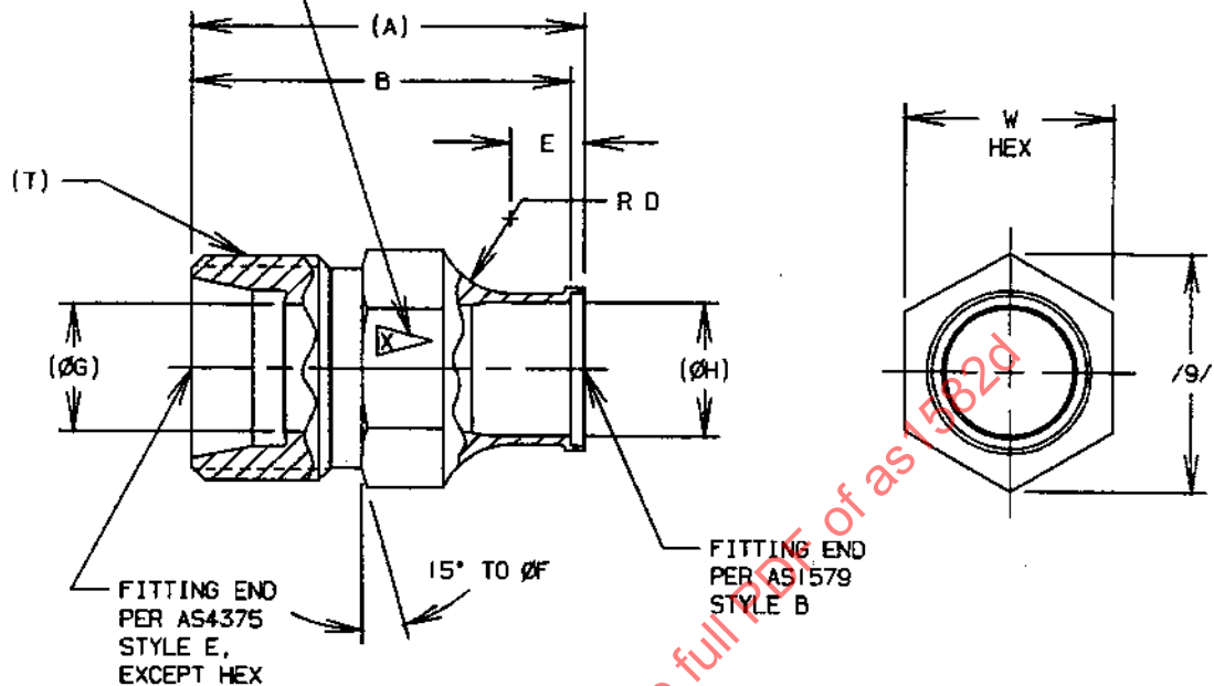
FIGURE 1 - FITTING, ADAPTER
