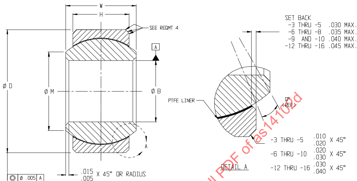
FIGURE 1 – PART CONFIGURATION
