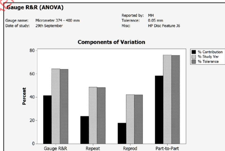
Figure 5 - Components of variation
