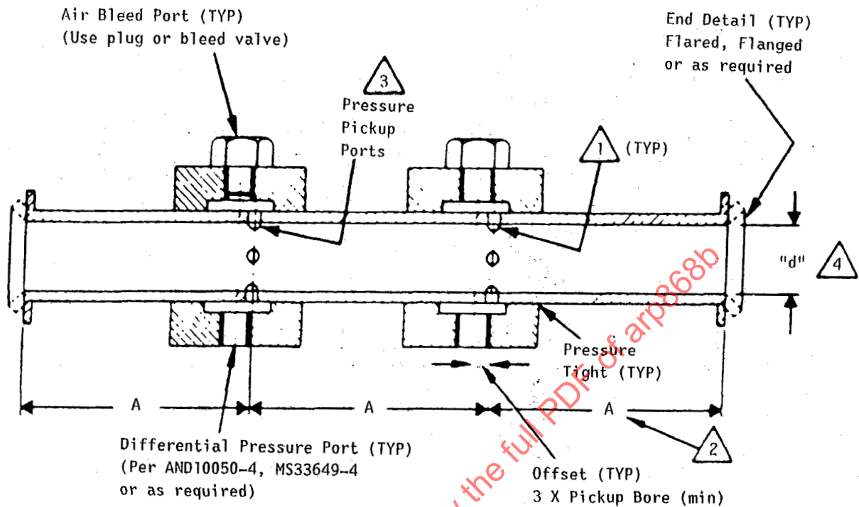
FIGURE 2 - Double Piezometer Tube
