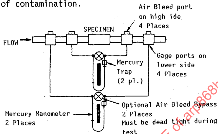
FIGURE 3 - Setup for Mercury Manometer
