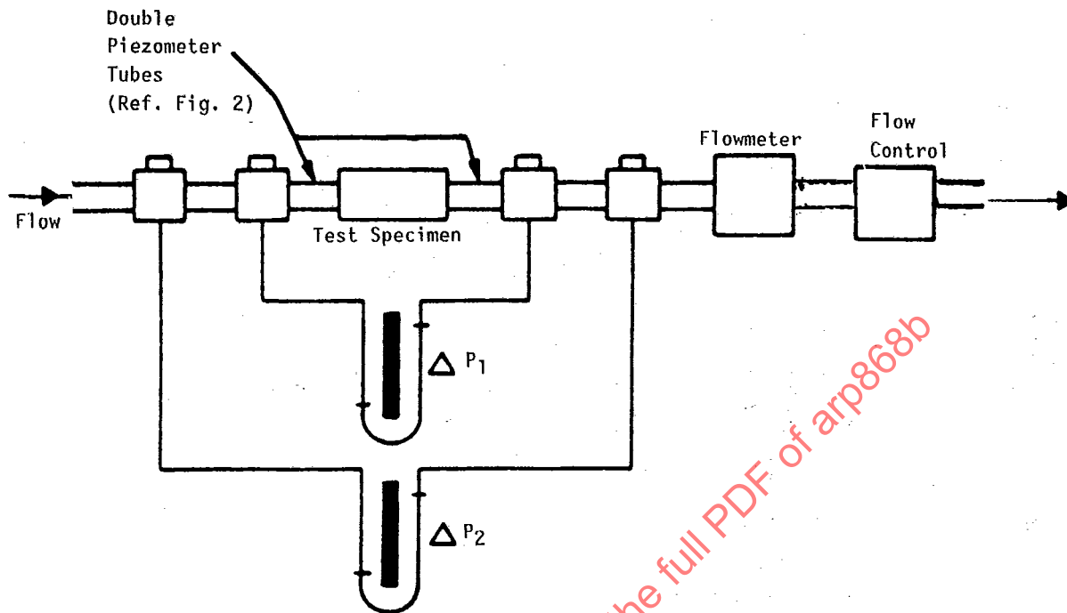
FIGURE 1 - Test Setup - Fuel Pressure Drop
