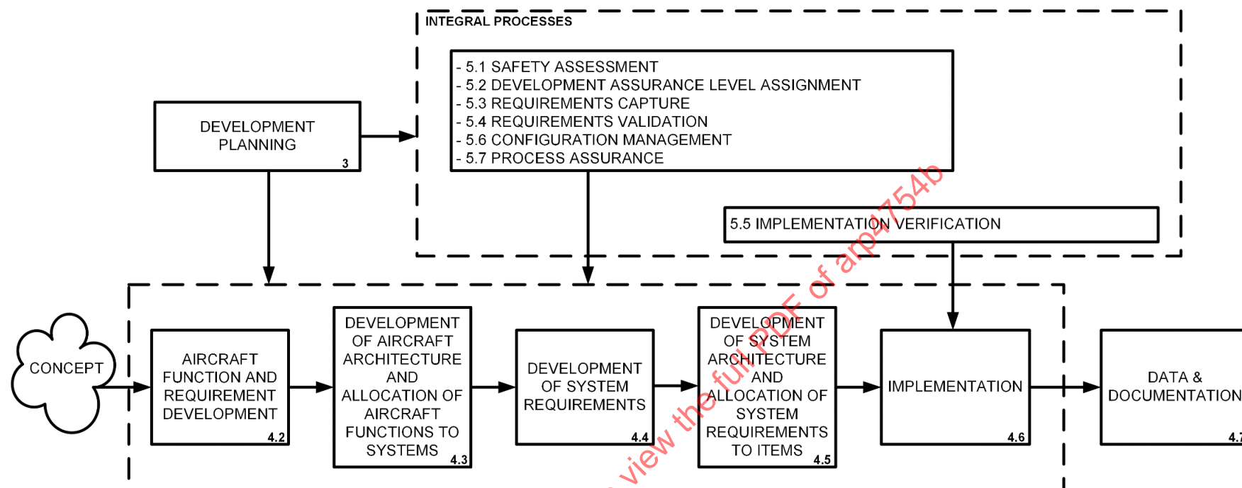
Figure 3 - Aircraft system development process
