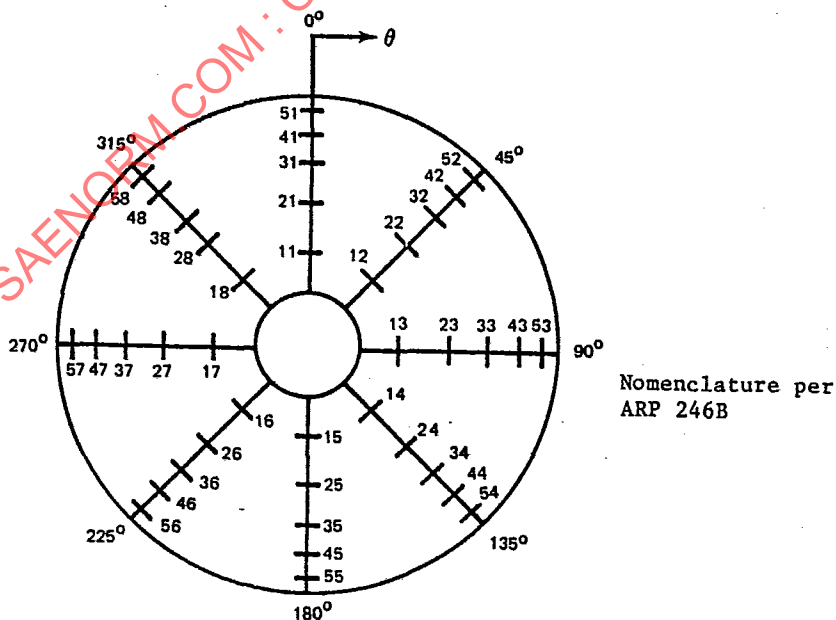
Figure 2 Probe Orientation - View Looking Forward
