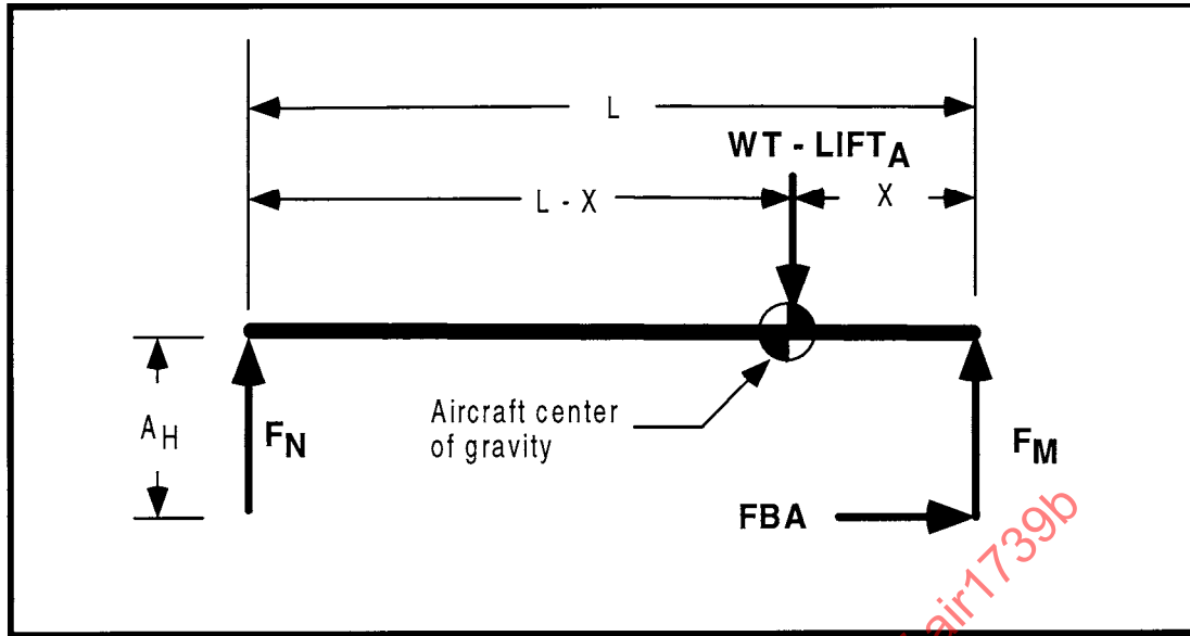
FIGURE 20 - AIRCRAFT LANDING GEAR GEOMETRY
