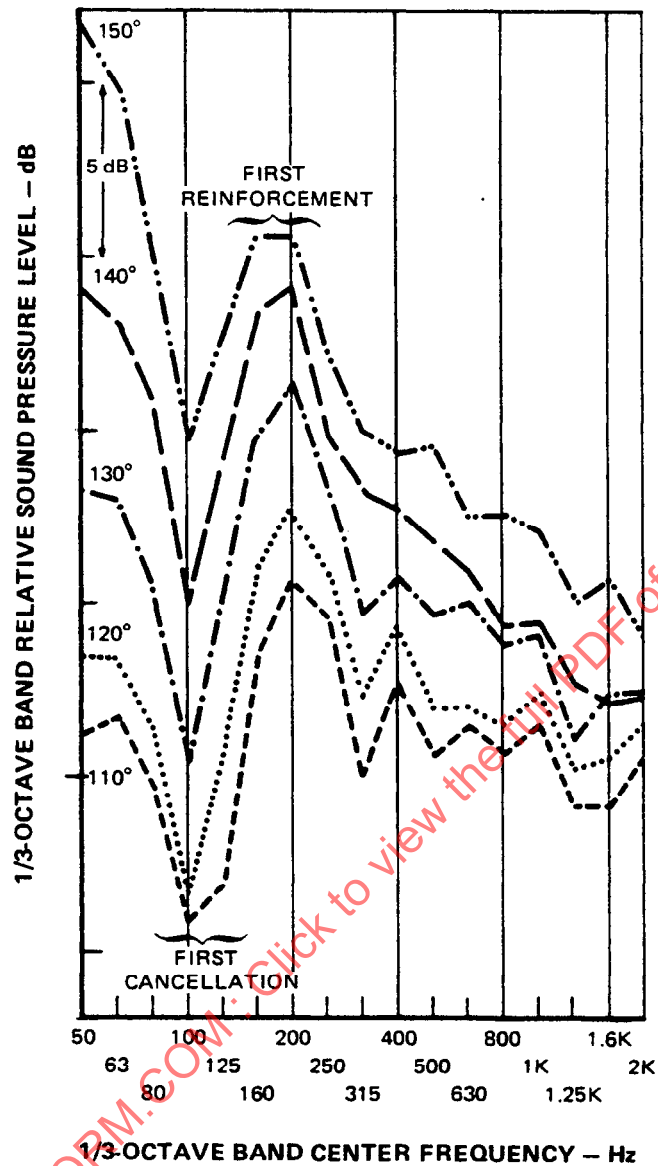
Figure C6 Spectra Measured at Aft Angles Over a Crushed Stone Surface at the P&WA Test Facility
