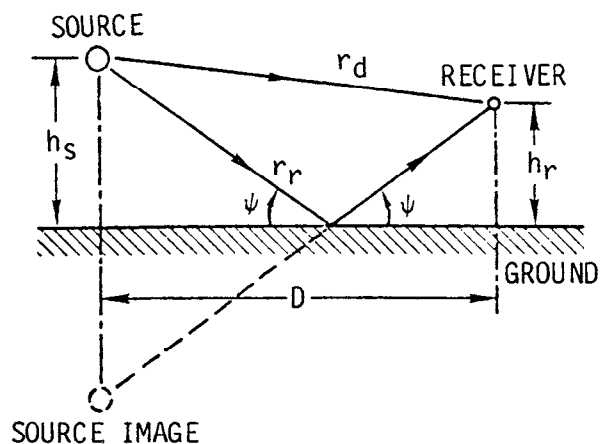
Figure C2 Geometry of Source and Receiver With Respect to Reflecting Ground Surface
