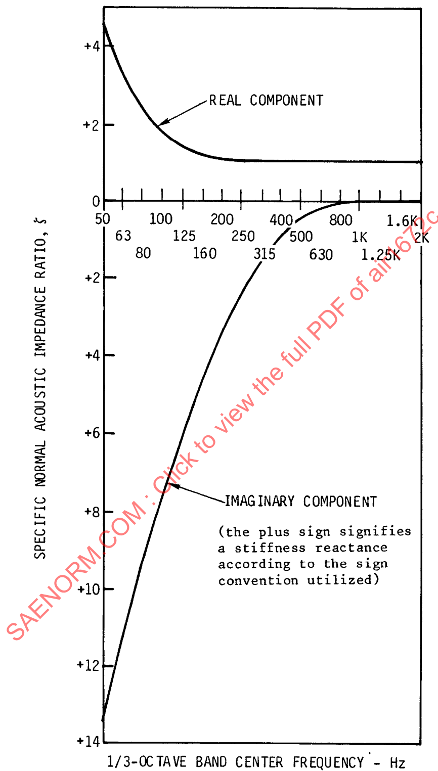
Figure C7 Specific Normal Acoustic Impedance Ratio for the Crushed Stone Surface at the P&WA Test Facility
