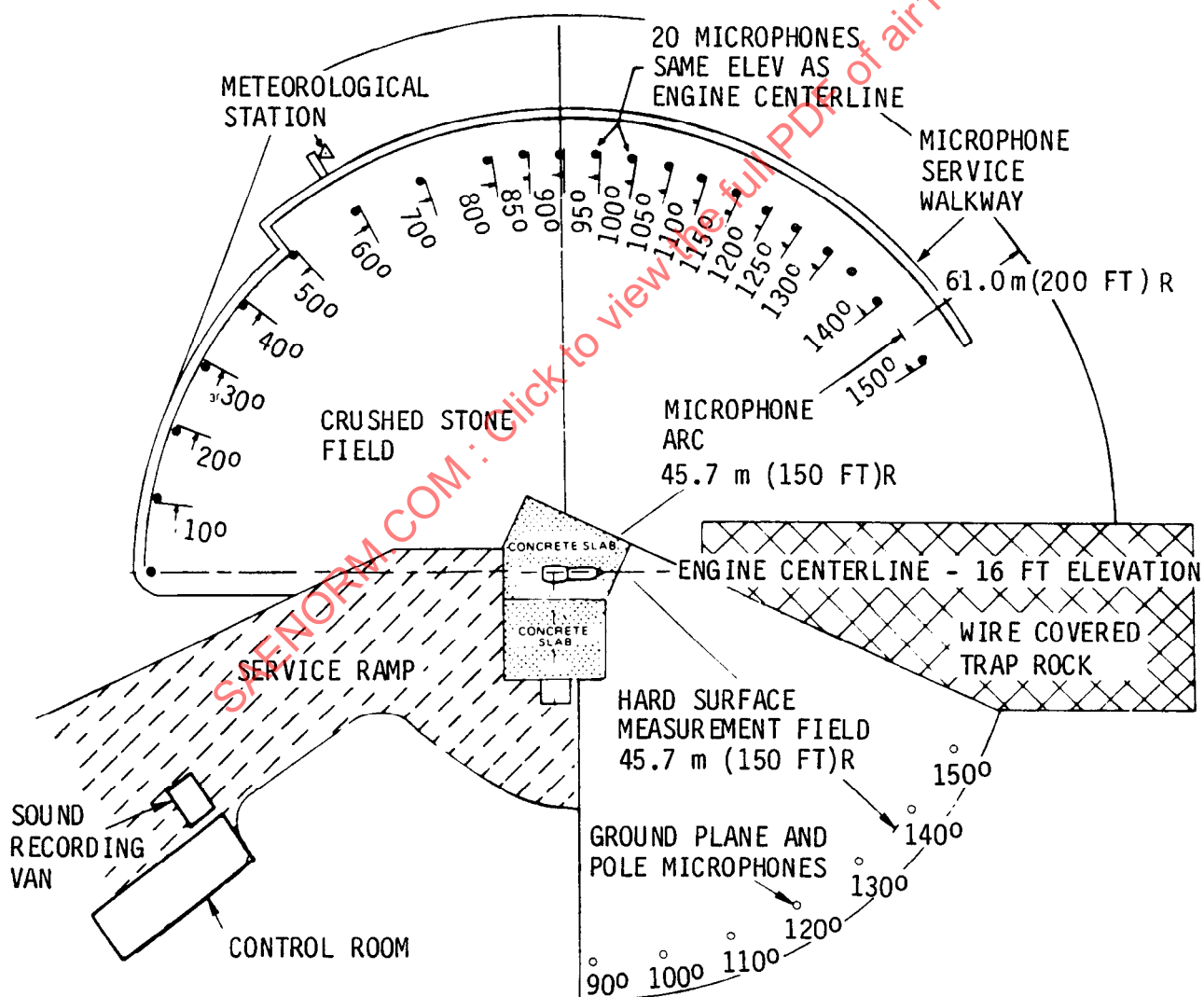
Figure C1 Pratt & Whitney Aircraft Outdoor Engine Noise Test Facility
