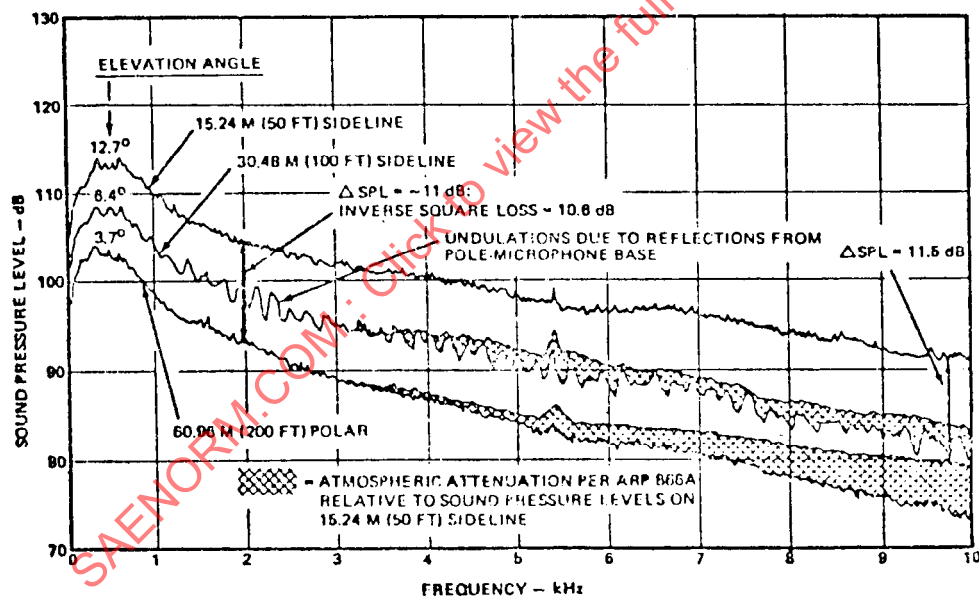
(b) MICROPHONES AT 120 DEGREES FROM ENGINE INLET AXIS
