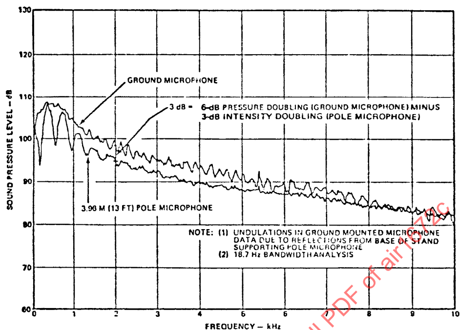
(a) MICROPHONES AT 120 DEGREES FROM ENGINE INLET AXIS
