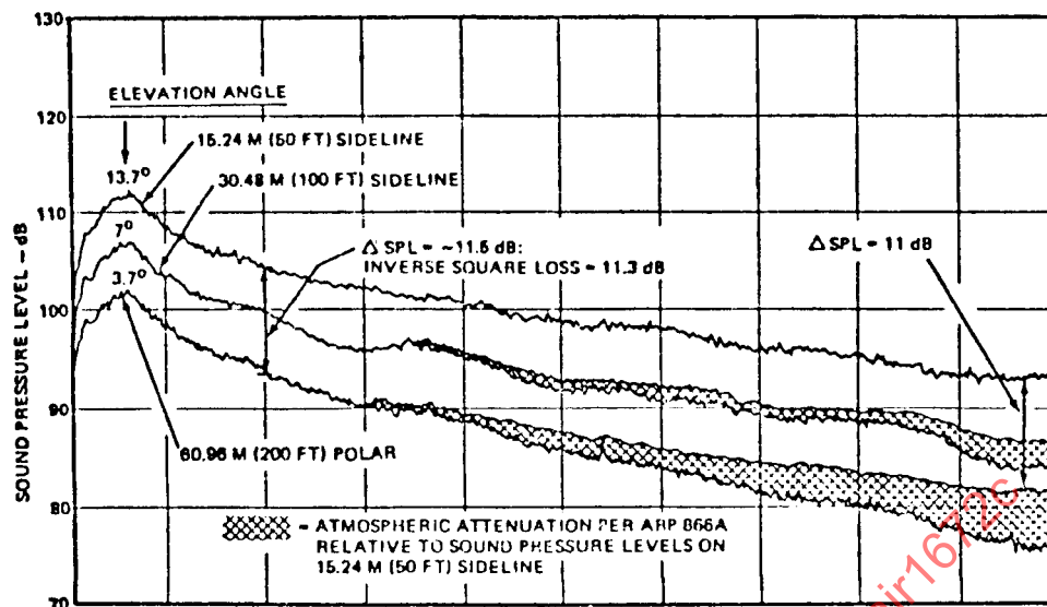
(a) MICROPHONES AT 110 DEGREES FROM ENGINE INLET AXIS
