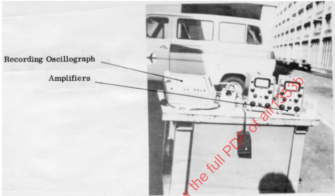
FIGURE 3. Test Instruments
