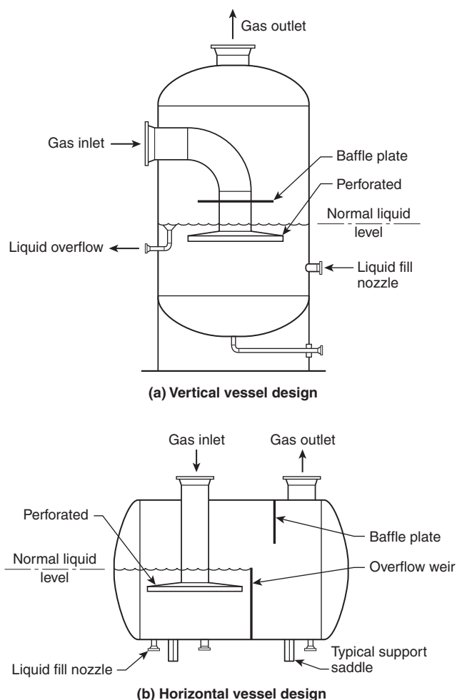
FIGURE A.12.2.5.1(a) Bubble Screen Hydraulic Flame Arrester.
