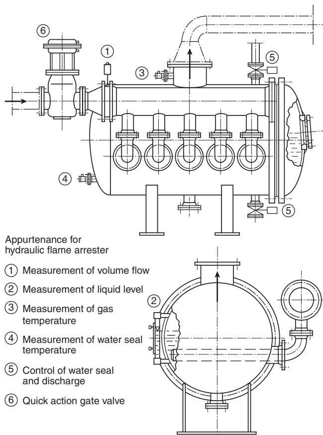
FIGURE A.12.2.5.1(b) Sparge Tube Hydraulic Arrester.
