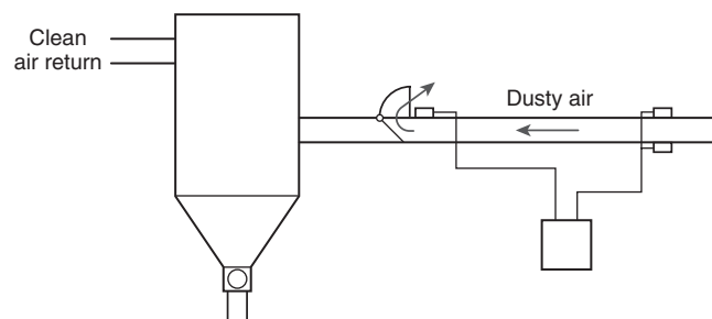
FIGURE A.8.2.2.6.4(a) Spark Detection and Abort Gate on Inlet Duct to the Dust Collector.
