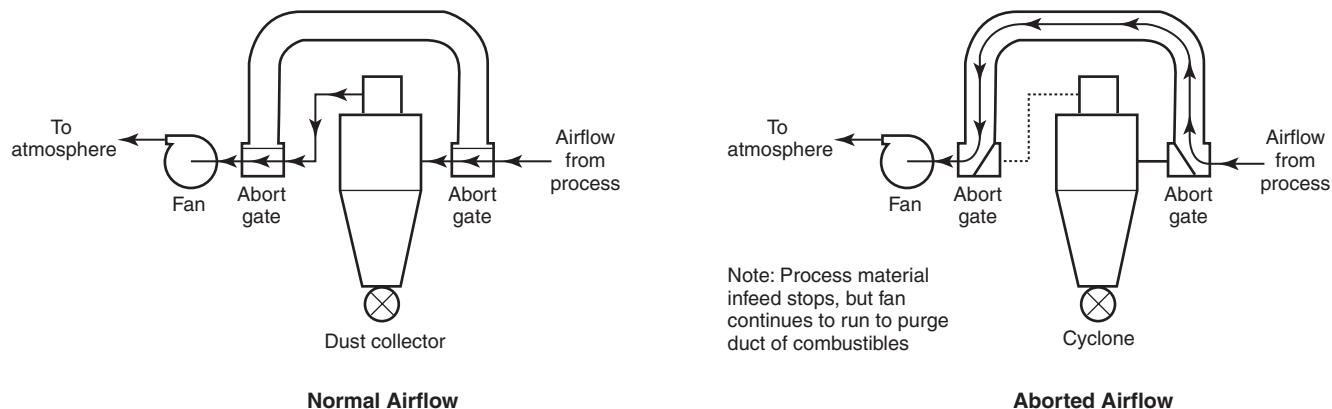
FIGURE A.8.2.2.2(2)(b) Aborting of Negative Pressure Systems.
