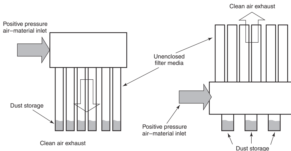
FIGURE A.3.3.10.2 Two Typical Enclosureless Dust Collectors.
