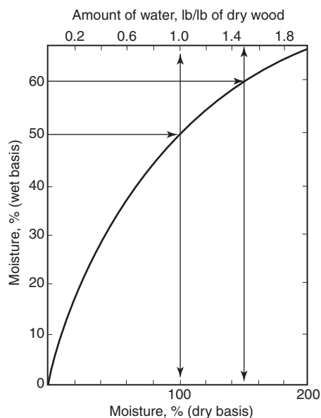
FIGURE A.3.3.18 Conversion from Wet Basis to Dry Basis.
