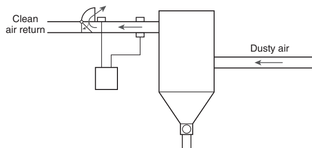
FIGURE A.8.2.2.6.4(b) Spark Detection and Abort Gate on Clean Air Side of the Dust Collector.
