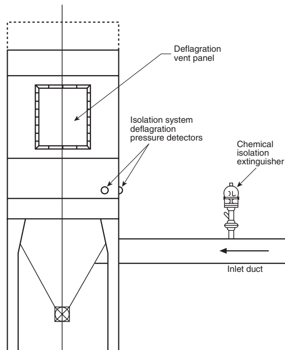
FIGURE B.4.4 Vented Dust Collector.
