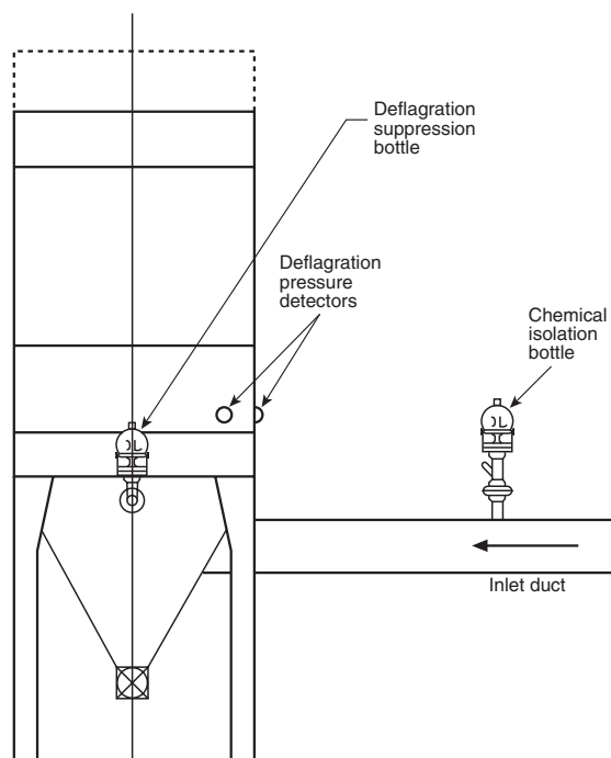
FIGURE B.5.2 Dust Collector Suppression System.
