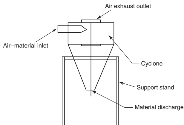
FIGURE A.3.3.9.1 A Typical Cyclone.
