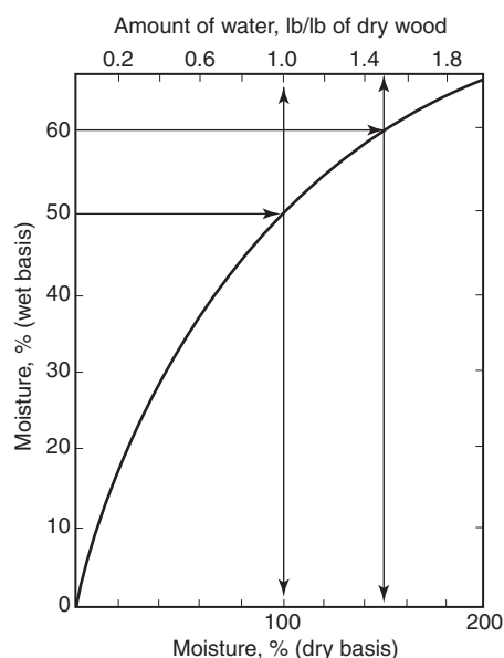
FIGURE A.3.3.14 Conversion from Wet Basis to Dry Basis.
