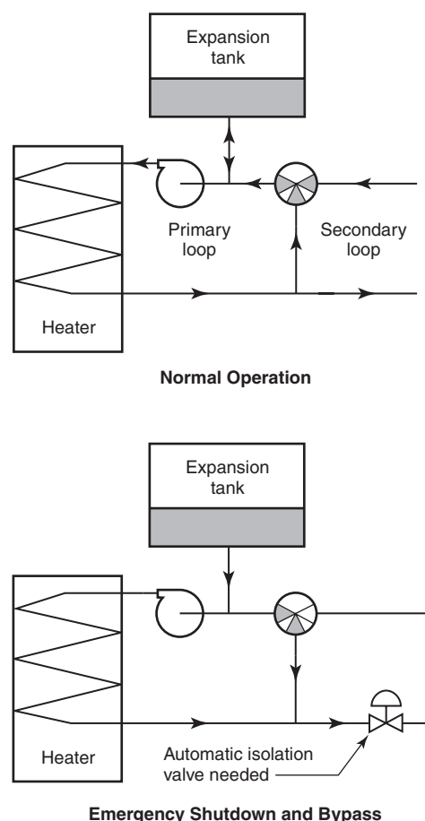
FIGURE A.8.3.1.1(5)(b) Three-Way Valve on Return Leg.
