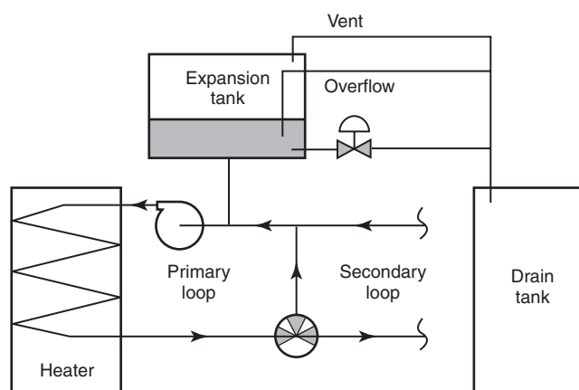
FIGURE A.8.3 Typical Thermal Oil System Components.
