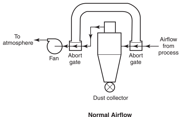
FIGURE A.8.2.2.2.2(b) Aborting of Negative Pressure Systems.
