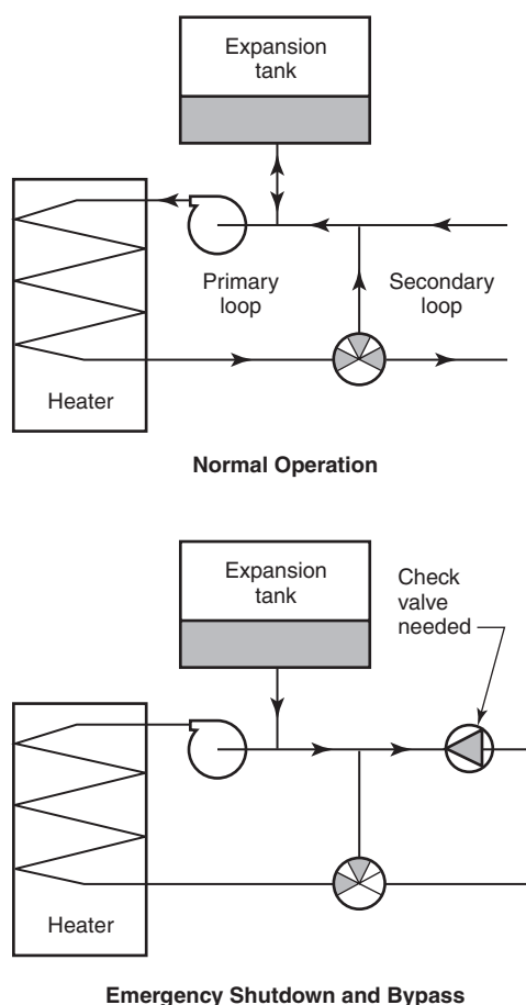
FIGURE A.8.3.1.1(5)(a) Three-Way Valve on Supply Leg.
