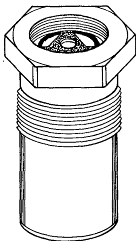
Sump Type Full Internal Relief Valve.
