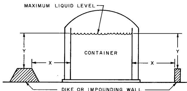
Figure 8-3.6 Dike or Impounding Wall Proximity to Containers.
