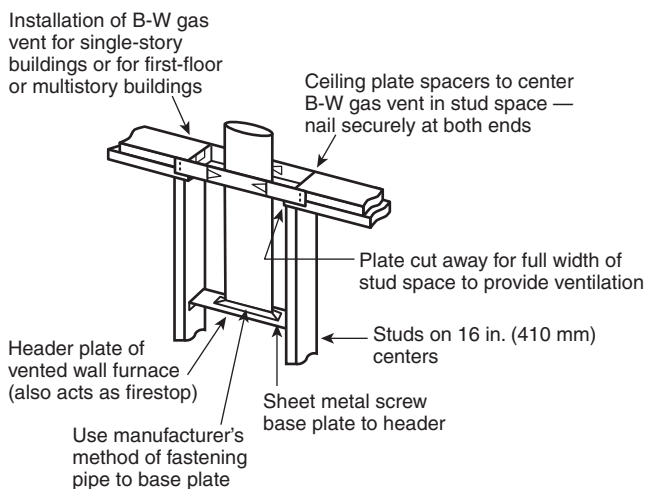
FIGURE 10.25.2.2 Installation of Type B-W Gas Vents for Vented Wall Furnaces.
