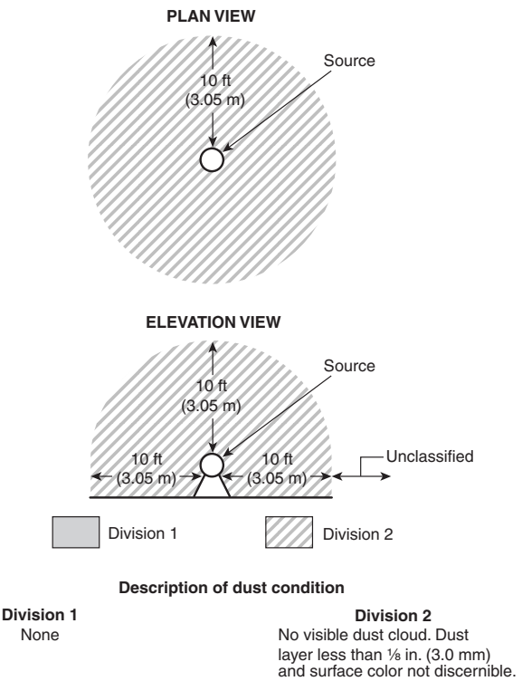
FIGURE 5.8(c) Group F or Group G Dust — Indoor, Unrestricted Area; Operating Equipment Enclosed; Area Classified as a Class II, Division 2 Location.
