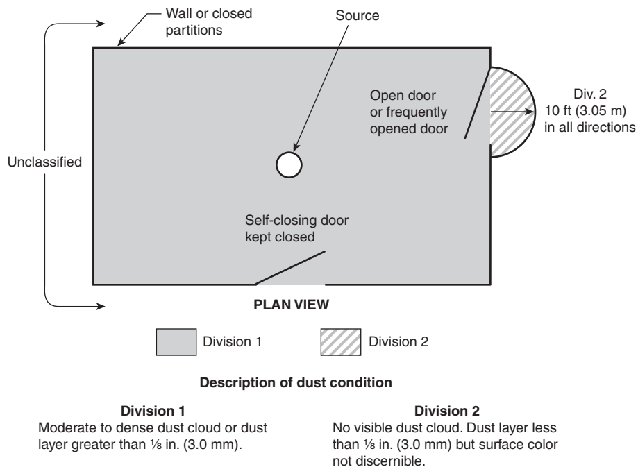
FIGURE 5.8(g) Group F or G — Indoor, Walled-Off Area; Operating Equipment Open or Semi-Enclosed.
