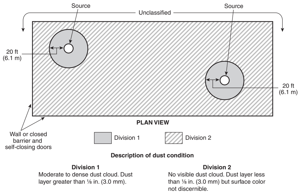
FIGURE 5.8(h) Group F or Group G — Indoor, Walled-Off Area; Multiple Pieces of Operating Equipment.
