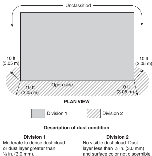
FIGURE 5.8(i) Group F or Group G — Indoor, Unrestricted Area; Ventilated Bagging Head.
