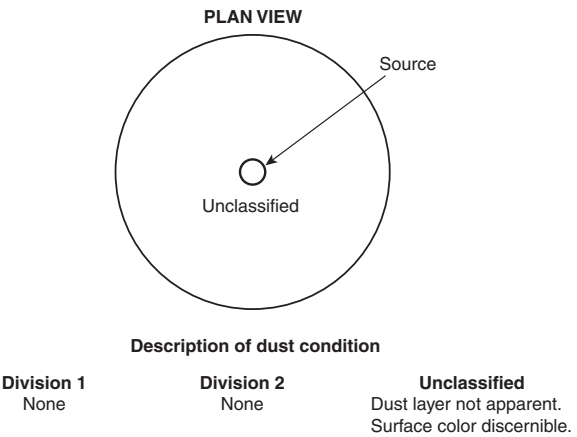
FIGURE 5.8(e) Groups E, F, or G Dusts — Storage Area Bags, Drums, or Closed Hoppers.
