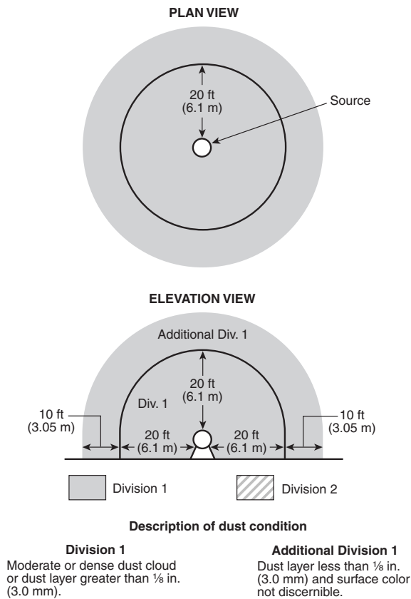
FIGURE 5.8(b) Group E Dust — Indoor, Unrestricted Area; Open or Semi-Enclosed Operating Equipment.
