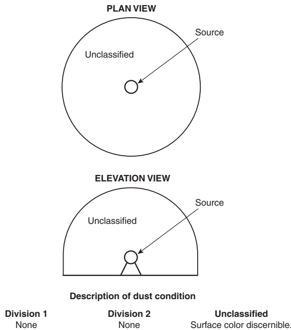
FIGURE 5.8(d) Group F or Group G Dust — Indoor, Unrestricted Area; Operating Equipment Enclosed; Area is an Unclassified Location.
