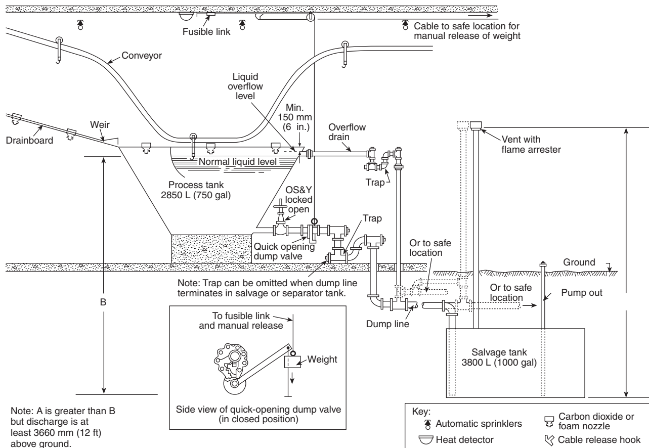
FIGURE C.1(c) Typical Process Tank Installation.
