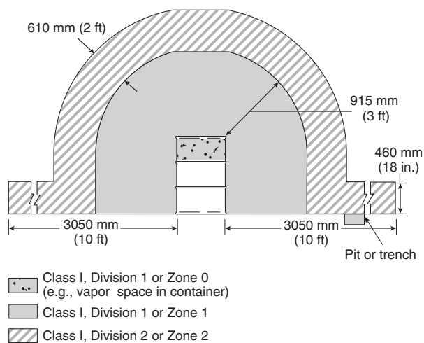
FIGURE 6.6 Electrical Area Classification around an Open Container in a Ventilated Area.
