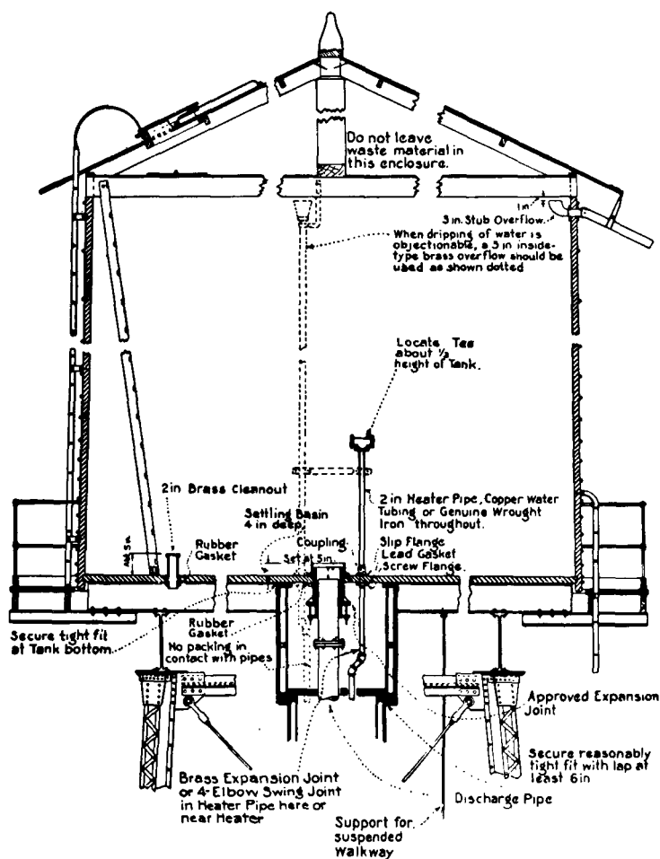
Fig. 10. Typical Tower-Supported Wood Tank.
