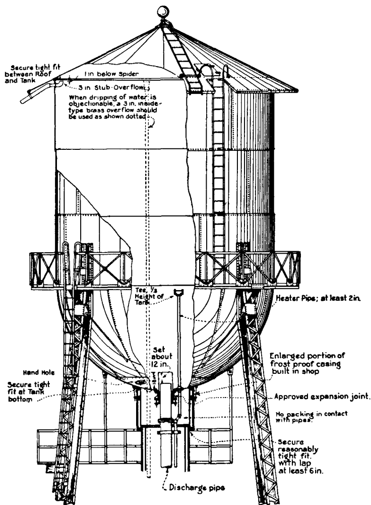
Fig. 11. Typical Tower-Supported Hemispherical-Bottom Riveted Steel Tank.
