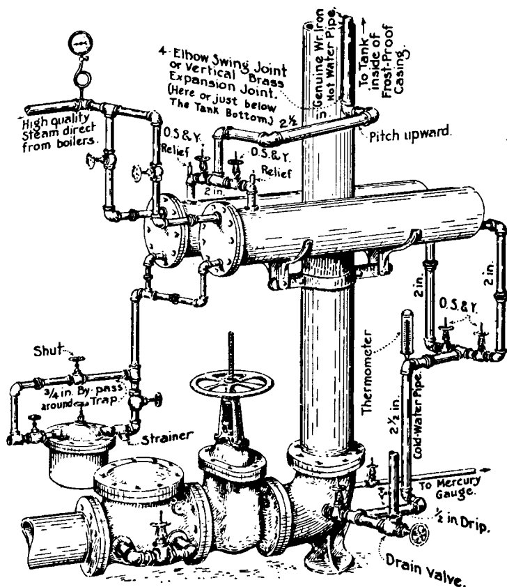
Fig. 15. Arrangement of Multiple Heaters.
