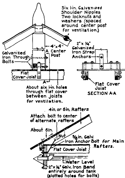
Fig. 5. Details of Tank Roof Construction.
