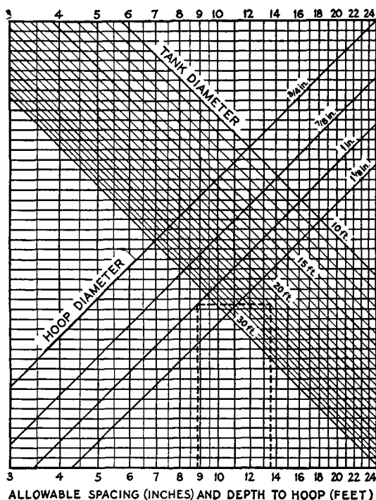
Fig. 3 Hoop Spacing Diagram for Wood Tanks.
