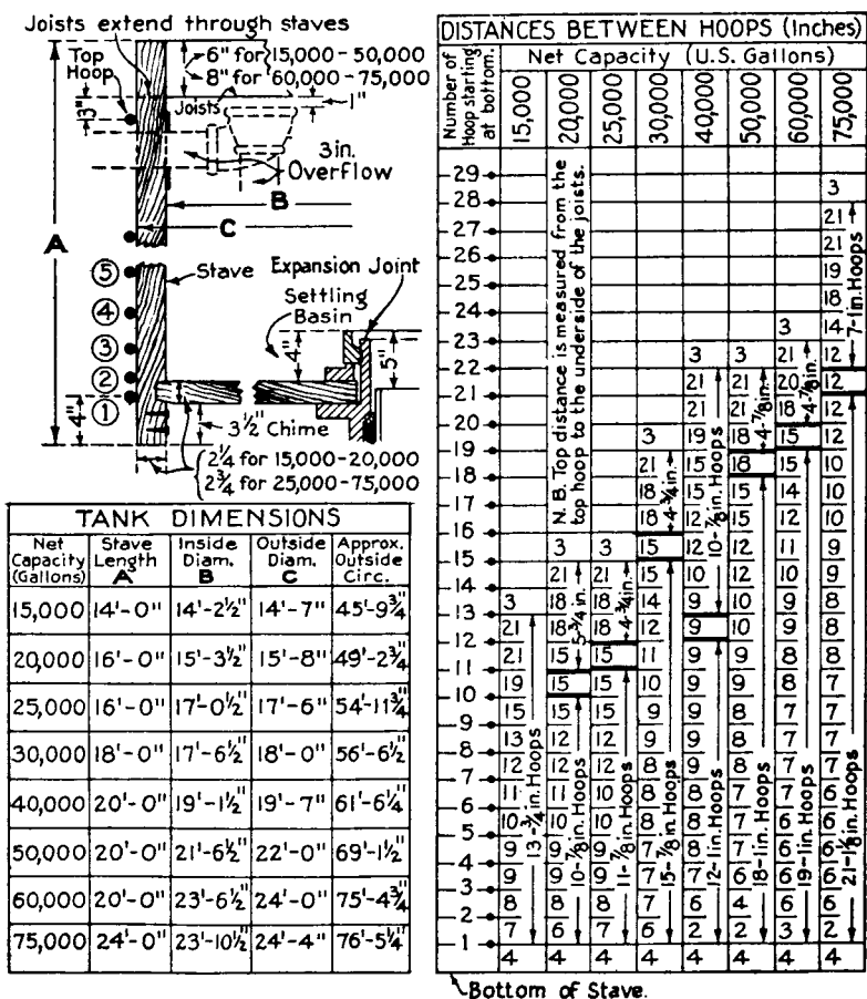
Fig. 2. Hoop Schedules for Wood Tanks. Dimensions are for cylindrical tanks.
