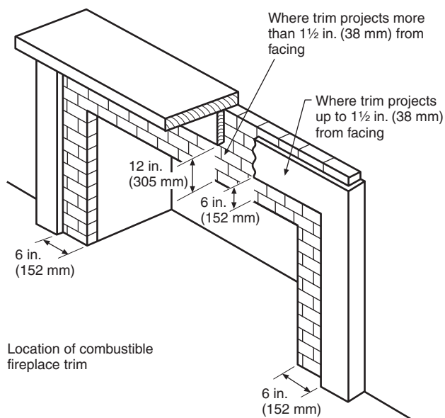
FIGURE 11.2.3.4 Fireplace Clearance to Combustible Material.
