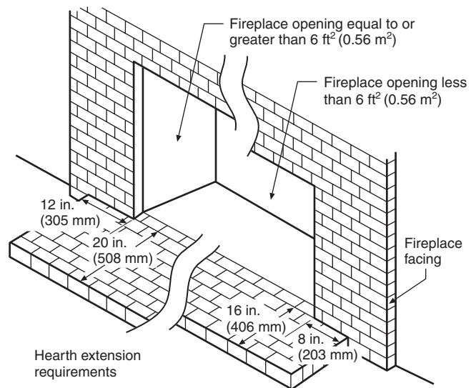
FIGURE 11.3.2 Fireplace Hearth Extension Details.
