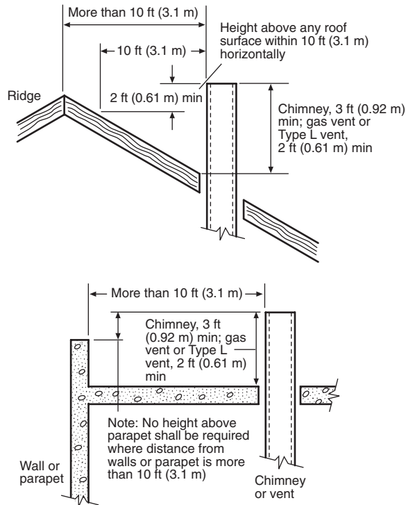
Figure 1-8.1(b) Chimney or vent termination [more than 10 ft (3.1 m)].
