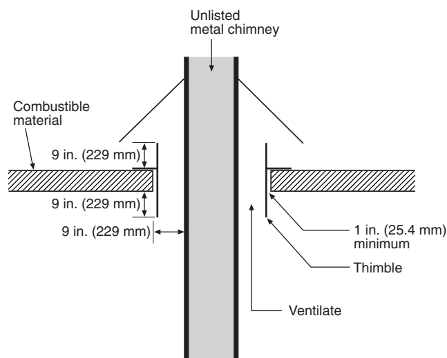
Figure 5-2.2.2.6 Ventilating thimble.
