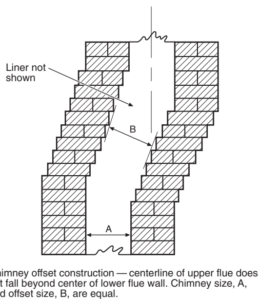
Figure 4-1.2(b) Corbels to change chimney direction.
