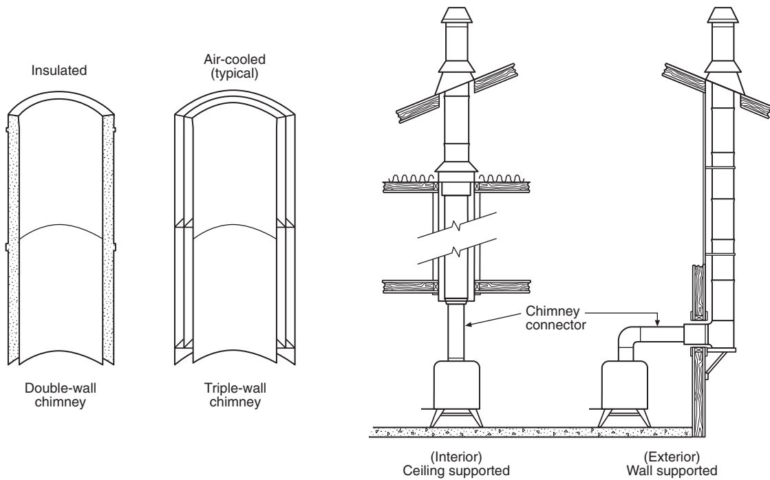
Figure 2-1(a) A typical factory-built chimney installation in a single-family residence; other applications can be determined by the chimney selection chart, Table 2-2.1.
