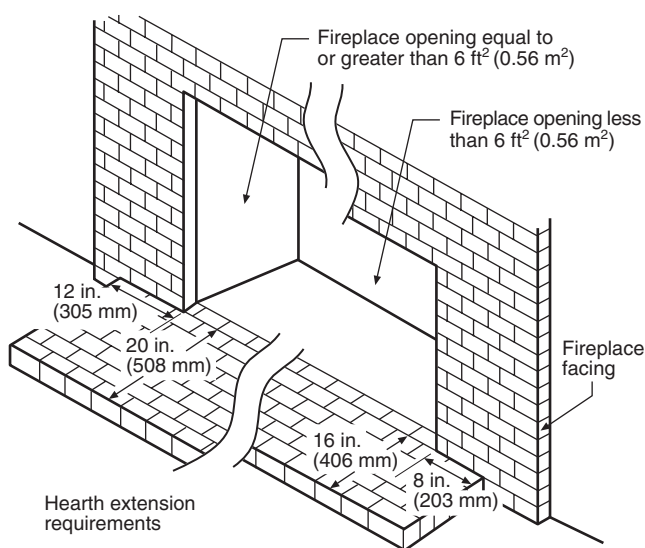
Figure 8-3.2 Fireplace hearth extension details.
