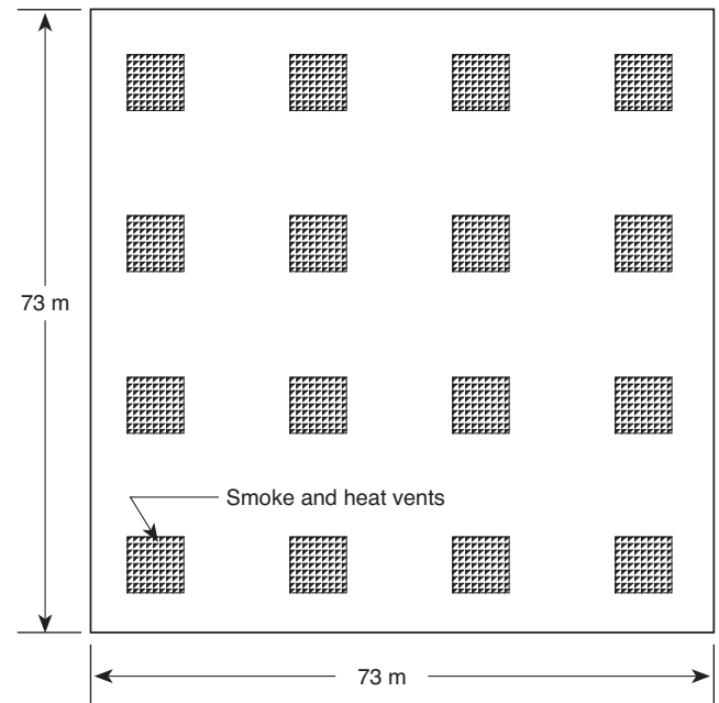
FIGURE D.2.3 Vent Plan View.
