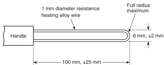
FIGURE 8.2.4.1 Wire Configuration.
