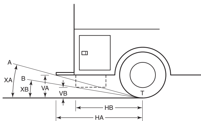
FIGURE A.5.7.1 Determination of Angle of Approach.
