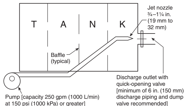
FIGURE A.18.5.2.2(a) Traditional Internal Jet Dump.
