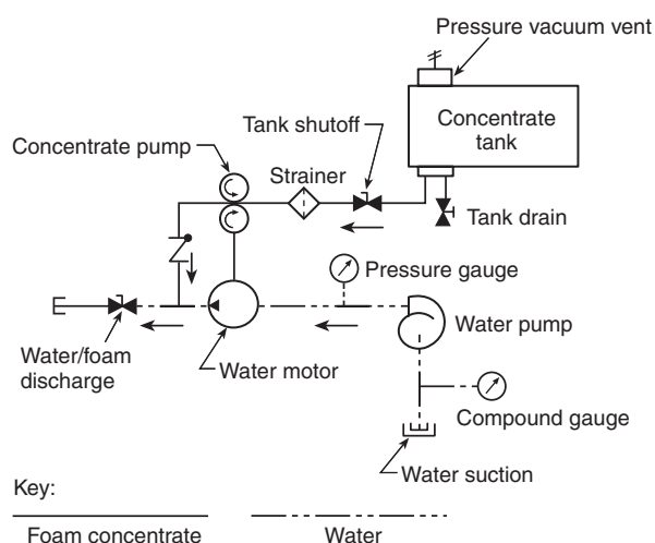
FIGURE A.20.2.7(a) Water Motor Foam Proportioning System.
