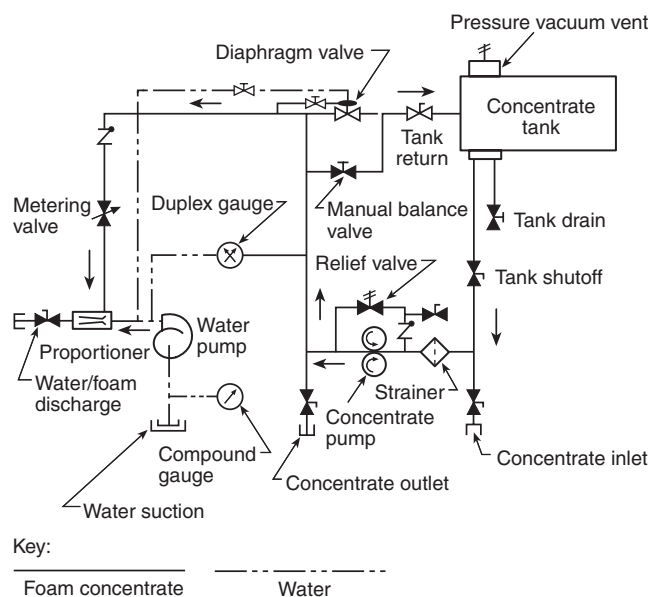
FIGURE A.20.2.5(b) Bypass Balanced Pressure Proportioning System.
