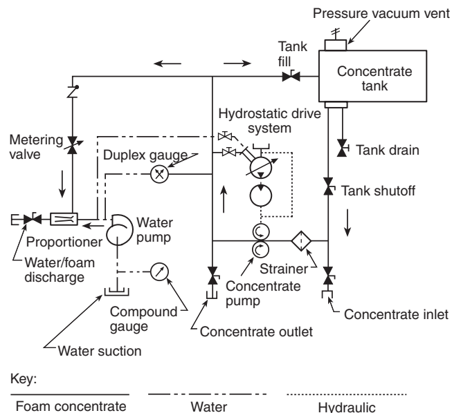
FIGURE A.20.2.5(c) Demand Balanced Pressure Proportioning System.
