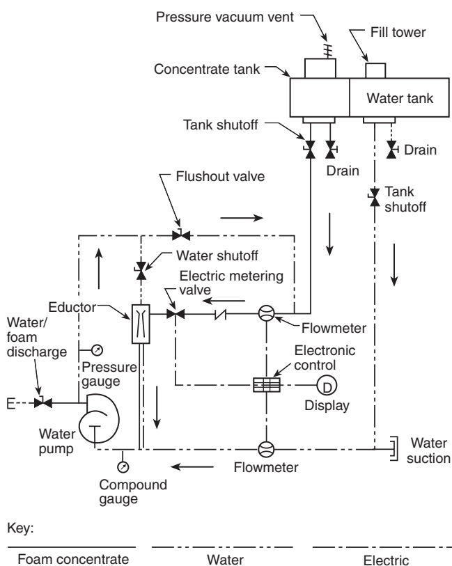
FIGURE A.20.2.4(b) Flowmeter Sensing Around-the-Pump Proportioning System.
