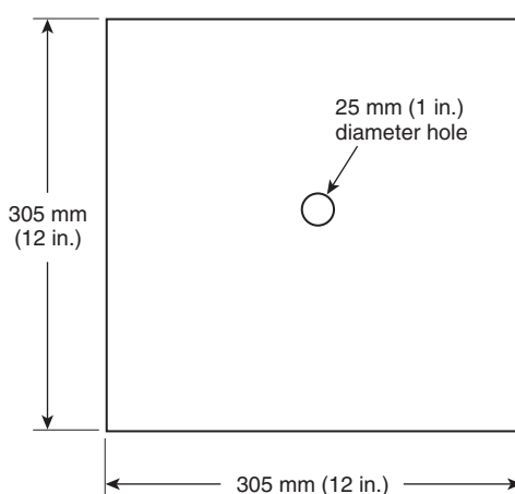
FIGURE 11.3.9.2 Hole Repairs.
