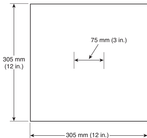
FIGURE 11.3.7.1 Tear Repairs.
