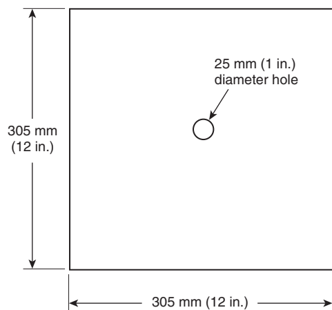
FIGURE 11.3.7.2 Hole Repairs.
