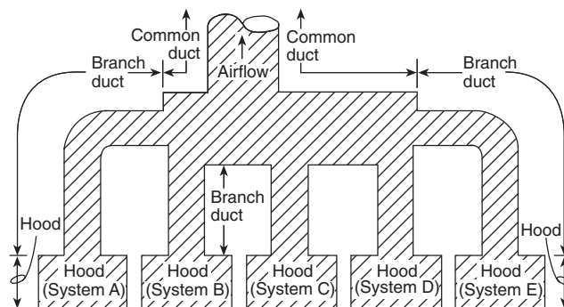
FIGURE A.9.3.4.1(1) Simultaneous Operation of All Systems.
