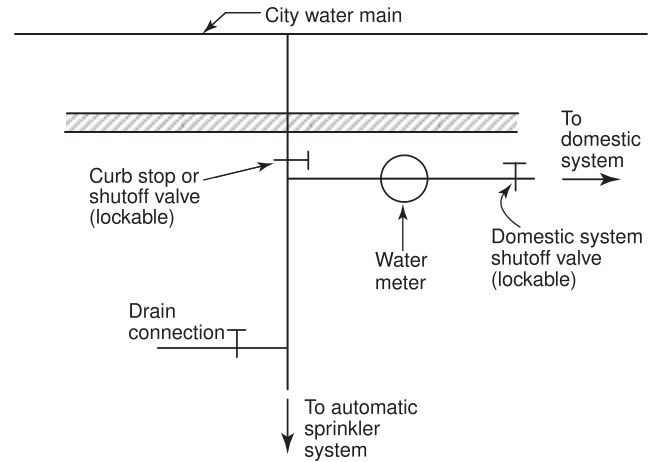
FIGURE A.6.2(a) Minimum Requirements for a Stand-Alone System.
