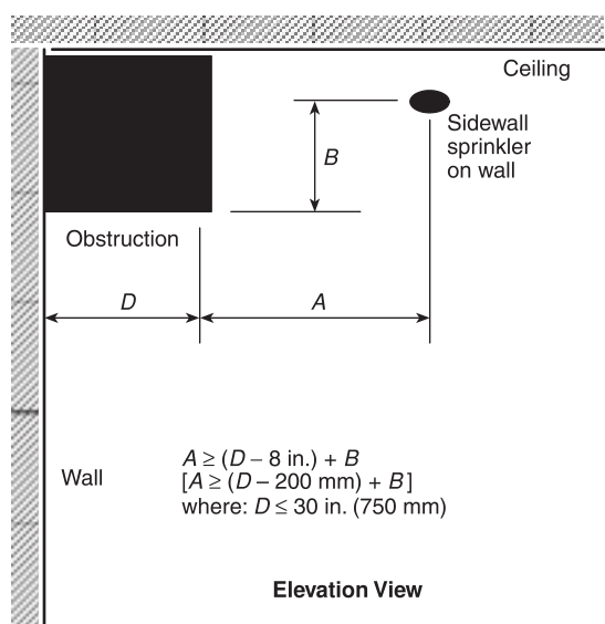
FIGURE 8.2.5.4.2(d) Positioning of Sprinkler to Avoid Obstructions Against Walls — Scenario 2 (Residential Sidewall Spray Sprinklers).
