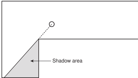
FIGURE A.3.3.11 Shadow Area Created by a Wall.
