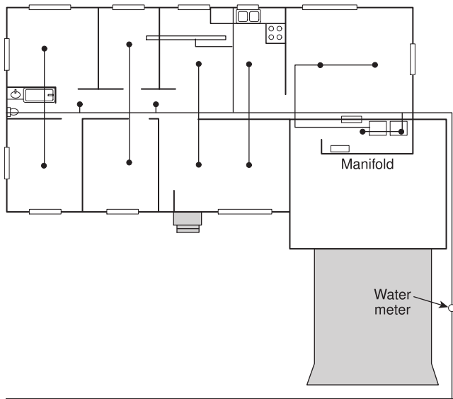
FIGURE A.3.3.13.3(a) Multipurpose Piping System (Tree System) — Example 1.
