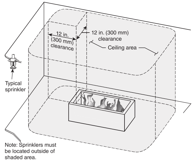
FIGURE A.7.5.6.3(3)(d) Open Fireplace — Intermediate Temperature Sprinkler Location.
