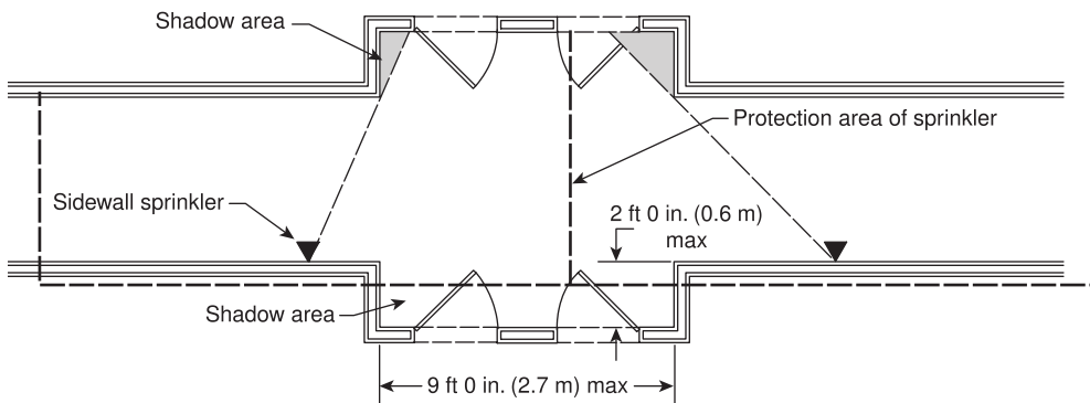
FIGURE 8.2.5.6 Shadow Areas Behind Sidewall Sprinklers in Corridors. [13R:Figure 6.4.6.3.3.2]
