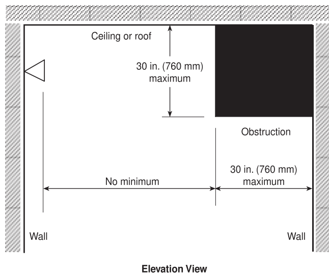
FIGURE 8.2.5.4.2(c) Positioning of Sprinkler to Avoid Obstructions Against Walls — Scenario 1 (Residential Sidewall Sprinklers).
