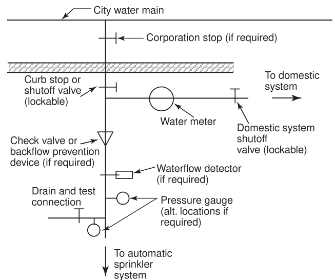
FIGURE A.6.2(b) Acceptable Arrangement for Stand-Alone Piping Systems — Option 1.
