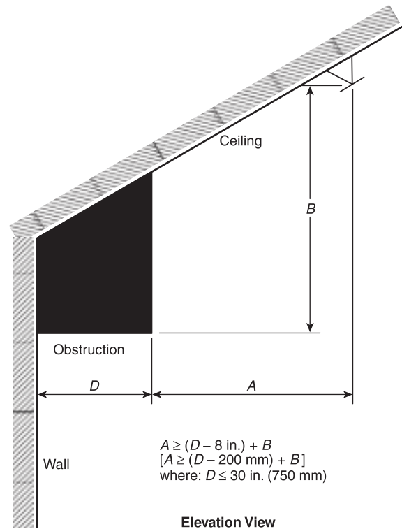
FIGURE 8.2.5.3.3(b) Positioning of Sprinkler to Avoid Obstructions Against Walls — Scenario 2 (Residential Upright and Pendent Spray Sprinklers).
