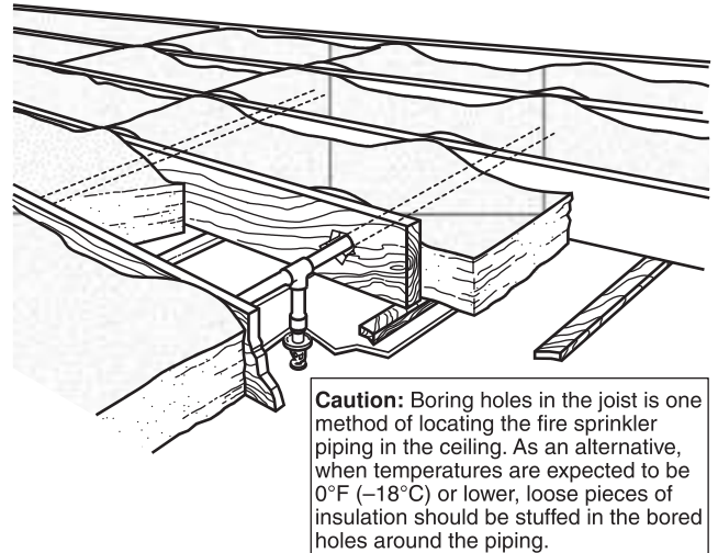
FIGURE A.9.1.1(c) Insulation Recommendations — Arrangement 3.
