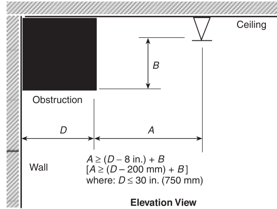
FIGURE 8.2.5.3.3(a) Positioning of Sprinkler to Avoid Obstructions Against Walls — Scenario 1 (Residential Upright and Pendent Spray Sprinklers).
