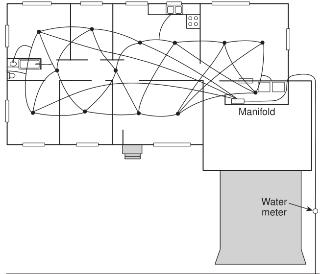
FIGURE A.3.3.13.3(c) Multipurpose Piping System — Example 3 (Network System).
