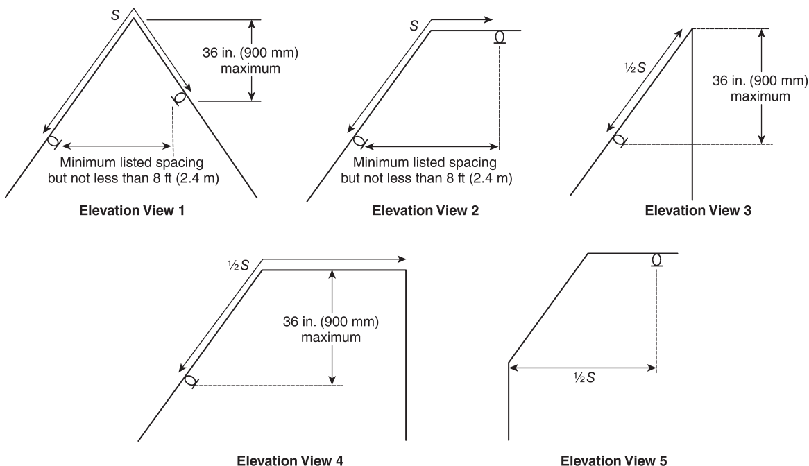
Δ FIGURE 8.1.1.1 Measuring S Dimension.
