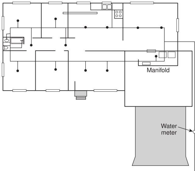
FIGURE A.3.3.13.3(b) Multipurpose Piping System (Looped System) — Example 2.
