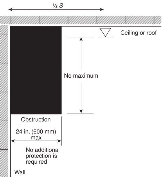
N FIGURE 8.2.5.3.3(c) Positioning of Sprinklers to Avoid Obstructions Against Walls — Scenario 3 (Residential Upright and Pendent Spray Sprinklers).
