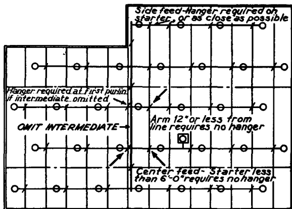
Fig. 3567. Hanger Omissions.
