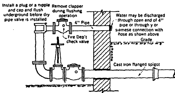
Employing fire department connections.
