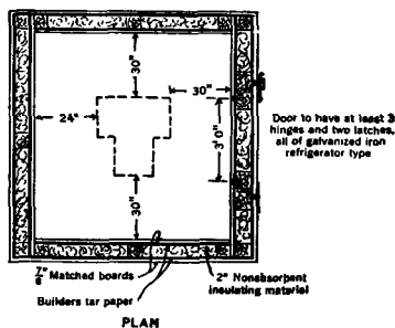
Fig. 5258-5. Dry-Pipe Valve Enclosure — Combustible Construction.
