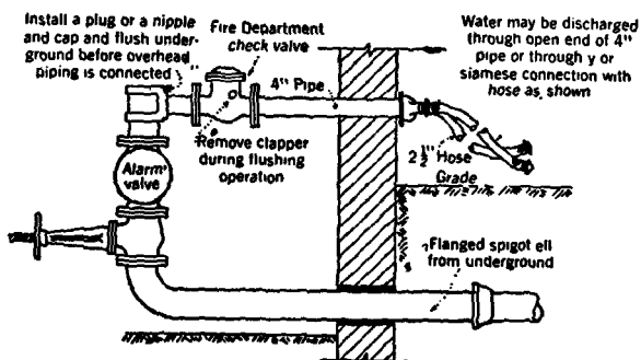
Employing horizontal run of 4-inch pipe and reducing fitting near base of riser.
