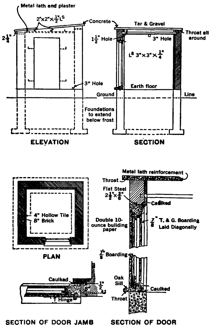
Fig. 5258-1. Dry-Pipe Valve Enclosures — Fire-Resistive Construction, Located Outside of Building with no Direct Communication to Building.
