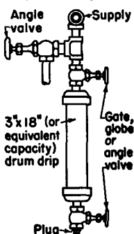
Fig. 3230. Auxiliary Drains.
