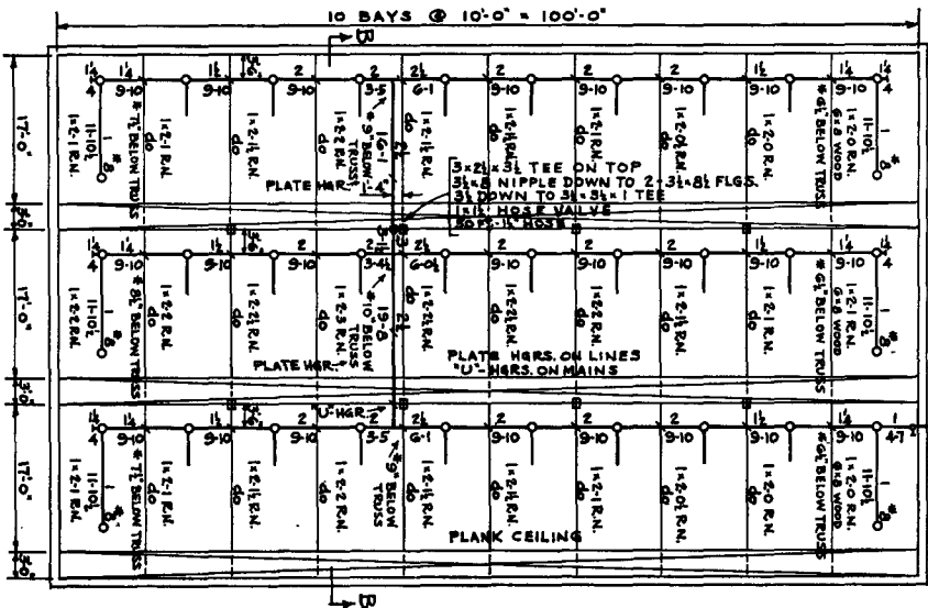
SECOND FLOOR OR ROOF PLAN
