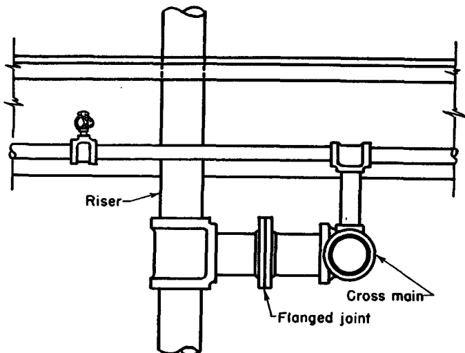
Fig. 3317. One Arrangement of Flanged Joint at Sprinkler Riser.
